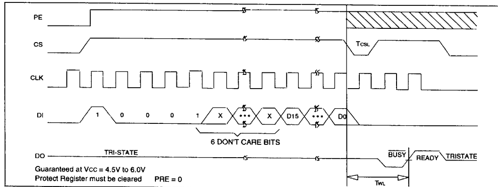
FIGURE 2-6: WRAL TIMING
