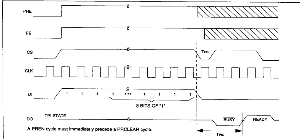
FIGURE 2-11: PRCLEAR TIMING
