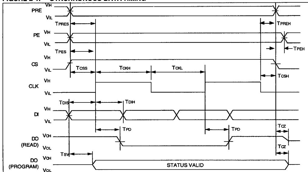
FIGURE 2-2: READ TIMING
