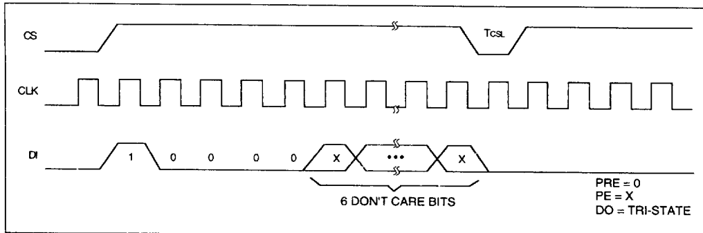
FIGURE 2-5: WRITE TIMING
