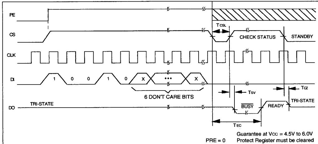
FIGURE 2-8: ERASE TIMING
