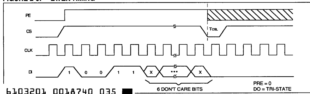
FIGURE 2-3: EWENTIMING
