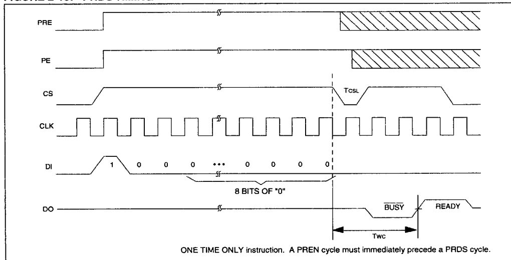
FIGURE 2-13: PRDS TIMING
