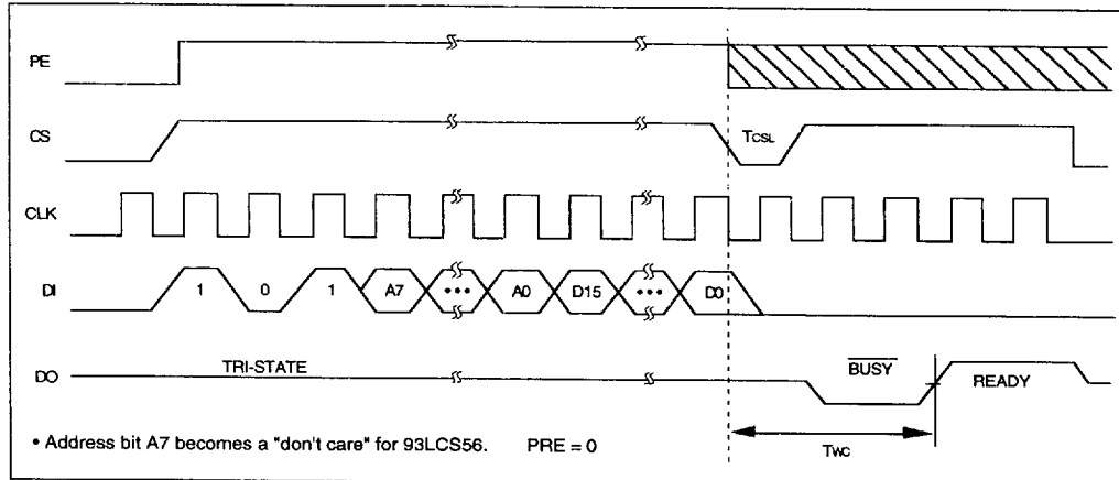
FIGURE 2-6: WRAL TIMING
