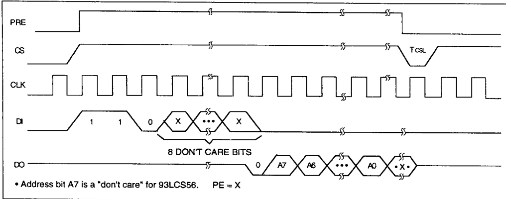
FIGURE 2-10: PREN TIMING
