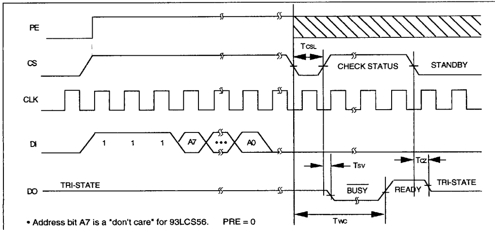
FIGURE 2-8: ERASE TIMING
