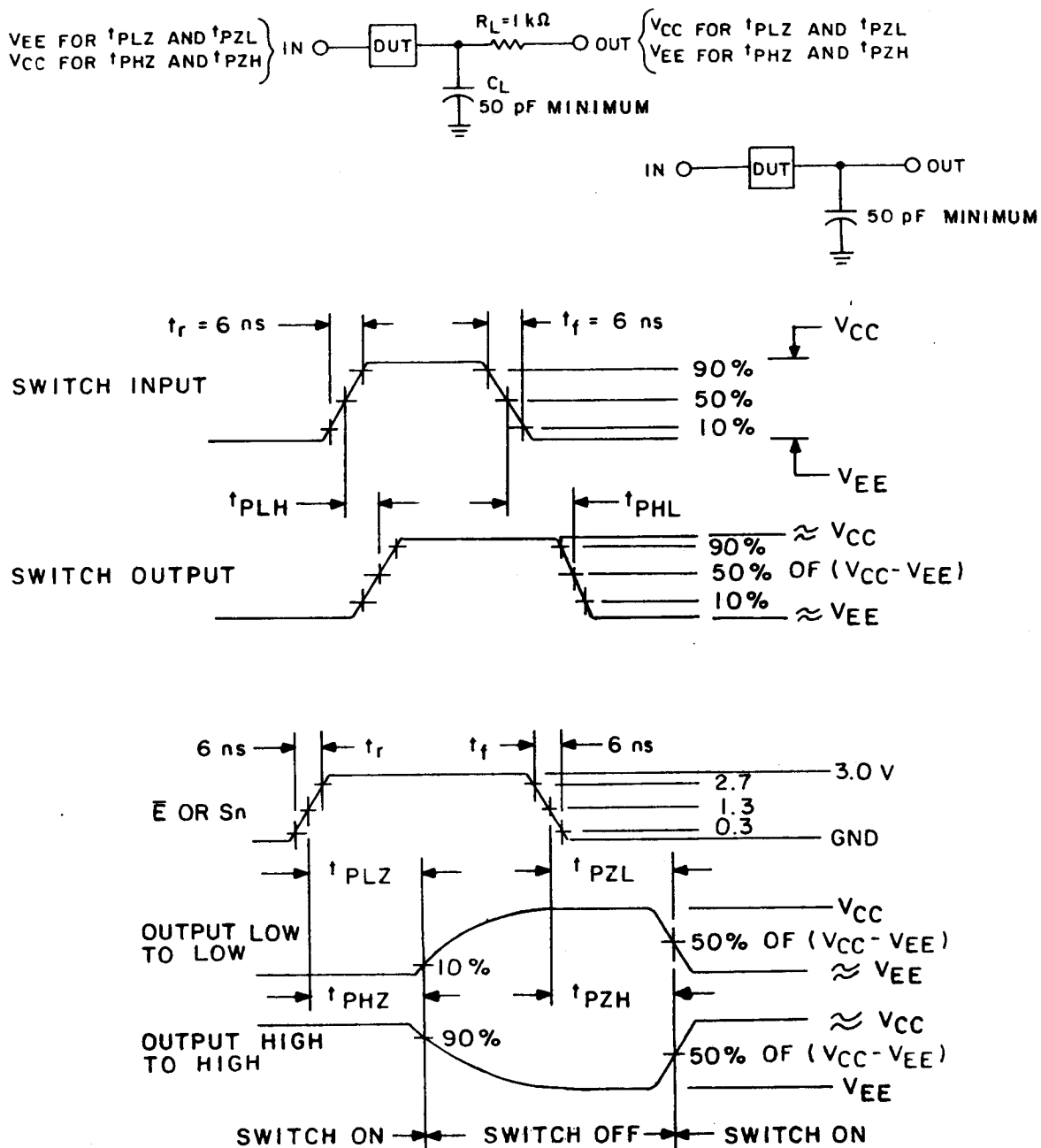
FIGURE 5. Test circuit and switching waveforms.
