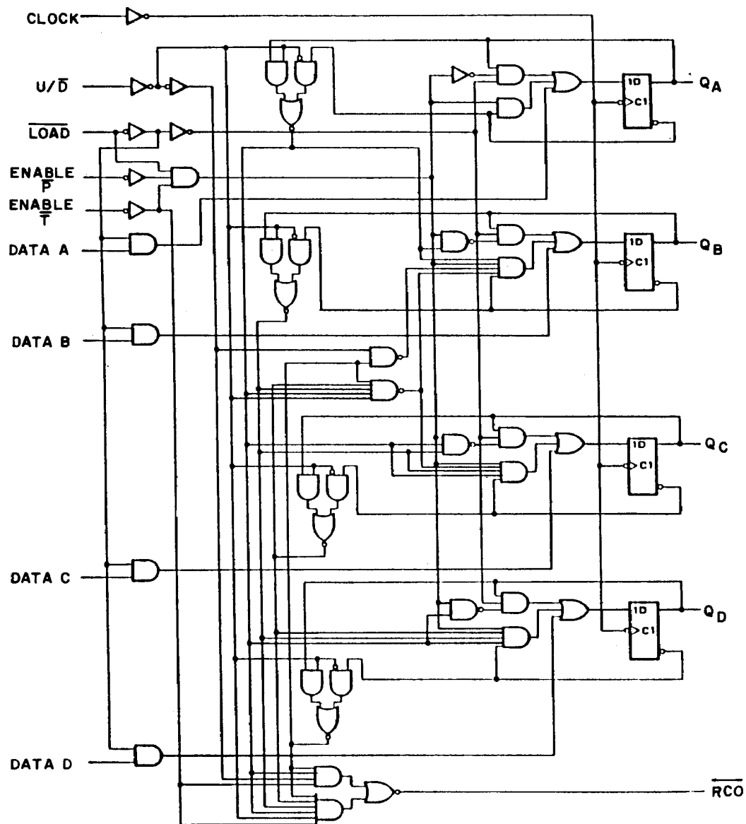
FIGURE 3. Logic diagram.
