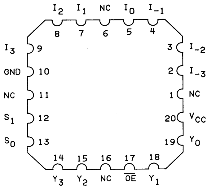
FIGURE 1. Terminal connections.
