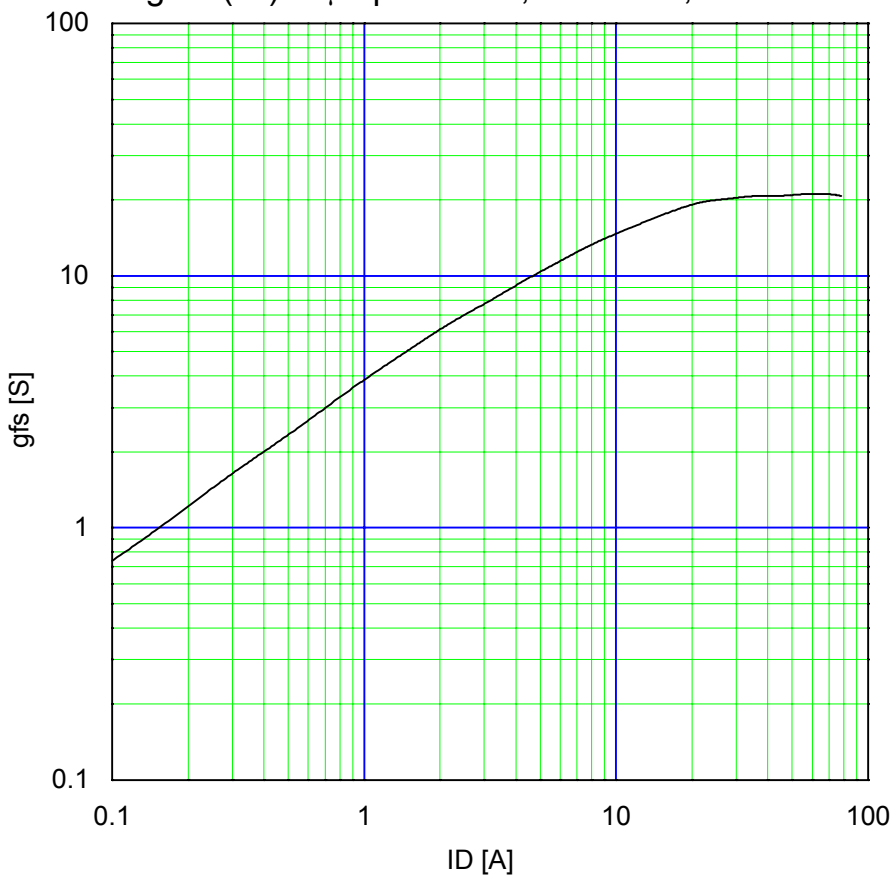
Typical Transconductance g_{fs}=f(I_D):80\mu s pulse test, V_{DS}=25V,T_{ch}=2^{\circ}C
