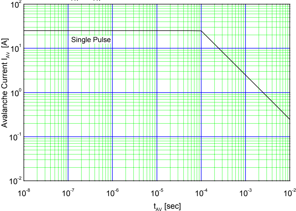
Maximum Avalanche Current Pulsewidth I_{AV}=f(t_{AV}): \text{starting Tch}=25^{\circ}\text{C}, V_{CC}=48V
