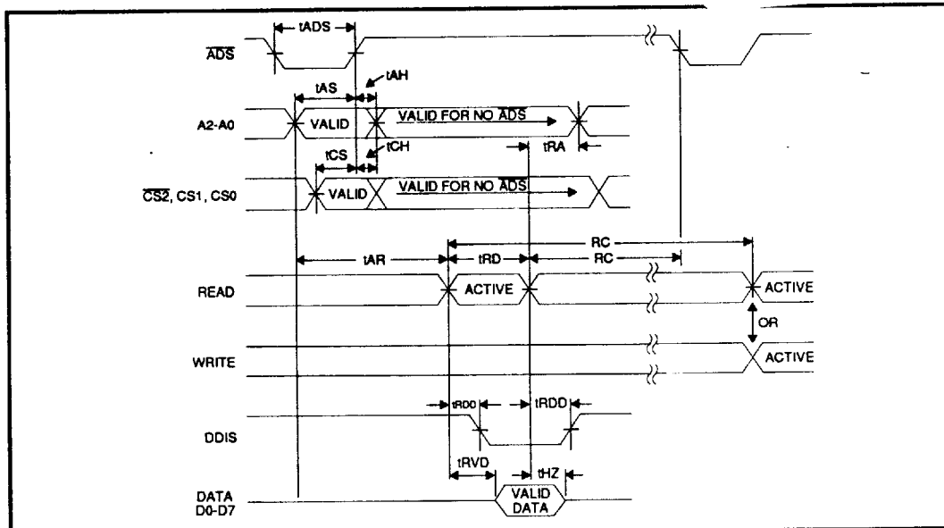
FIGURE 4: Read Cycle Timing
