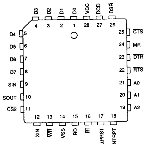
SSI 73M2550 UART 28-PIN PLCC
