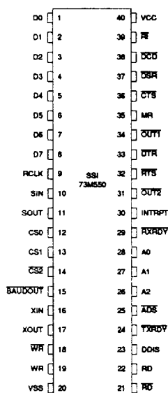
SSI 73M550/550F 40-Pin DIP
