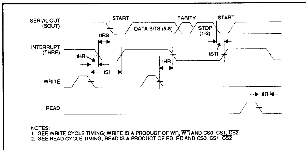
FIGURE 6: Transmitter Timing
