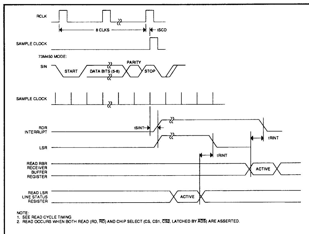
FIGURE 11: Receiver Timing
