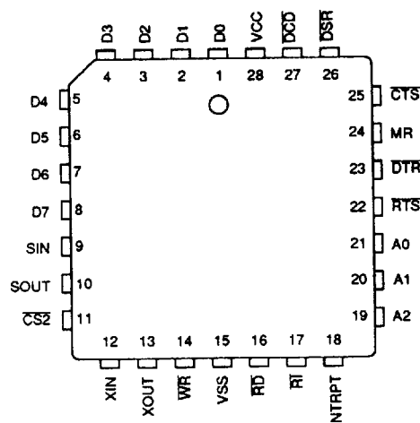
SSI 73M1550 UART 28-PIN PLCC
