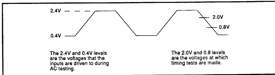
FIGURE 3: AC Test Points*
