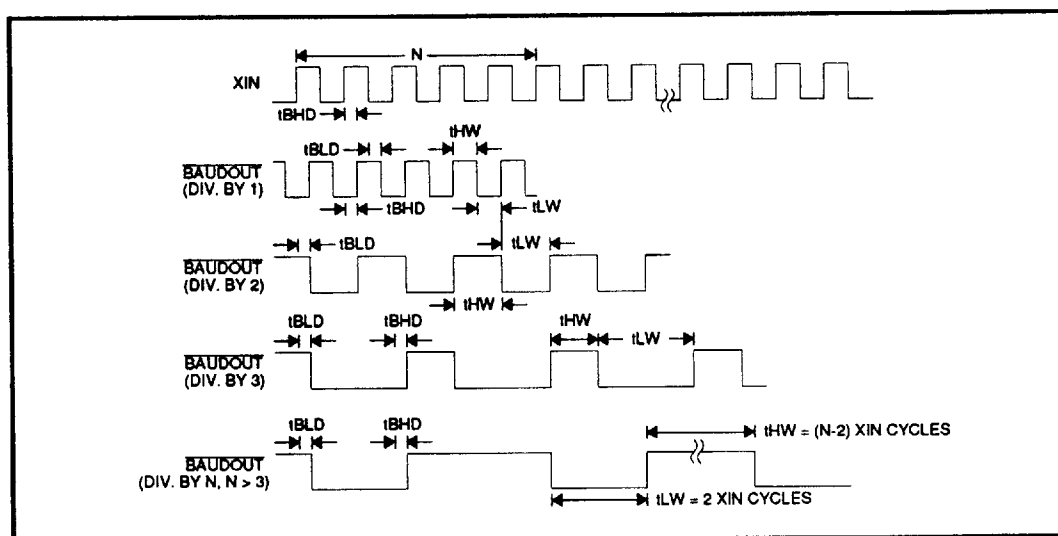
FIGURE 10: BAUDOUT Timing
