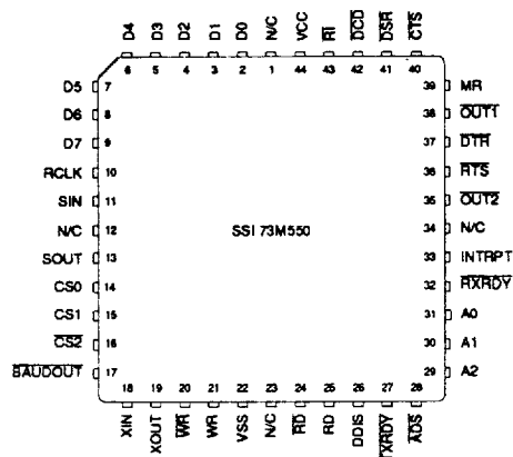
SSI 73M550/550F 44-Pin PLCC
