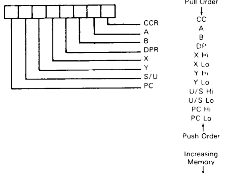
Push/Pull Postbyte
