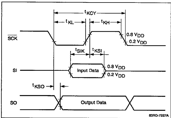
Figure 7. Serial Transfer Timing
