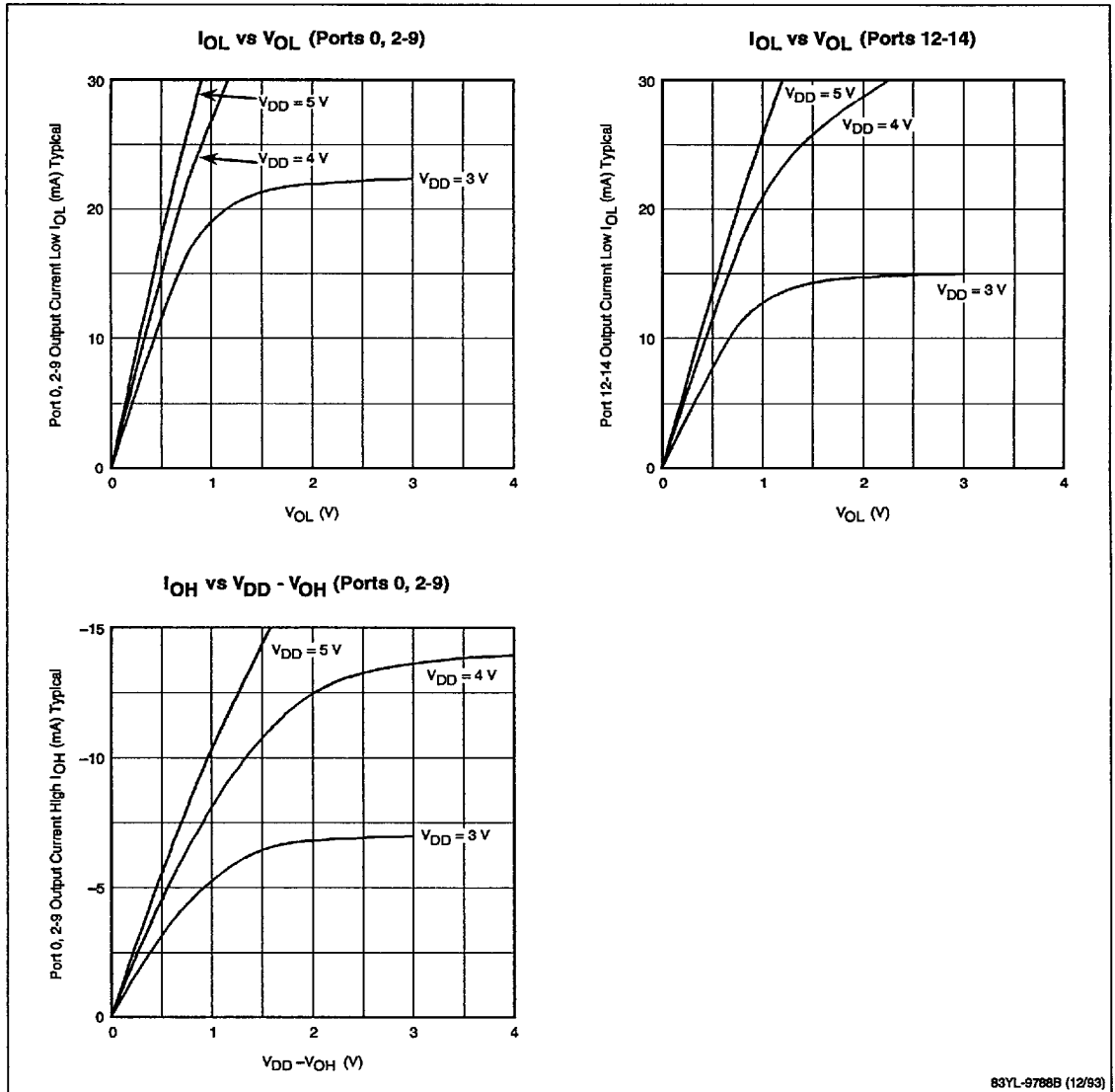
Figure 2. DC Characteristics (cont)
