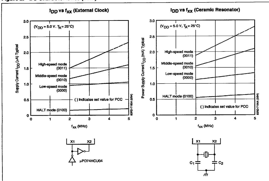
Figure 2. DC Characteristics (cont)
