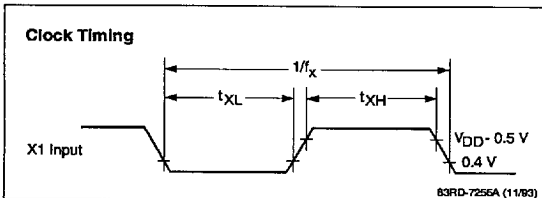
Figure 6. T1 Timing
