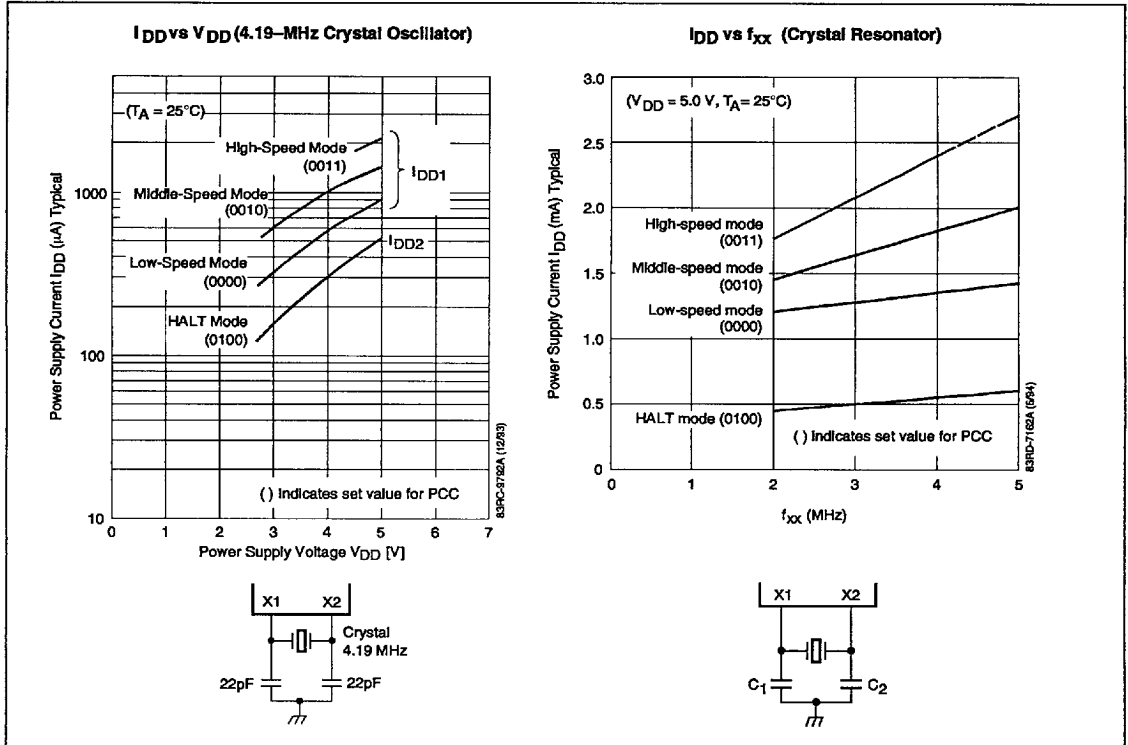
Figure 2. DC Characteristics
