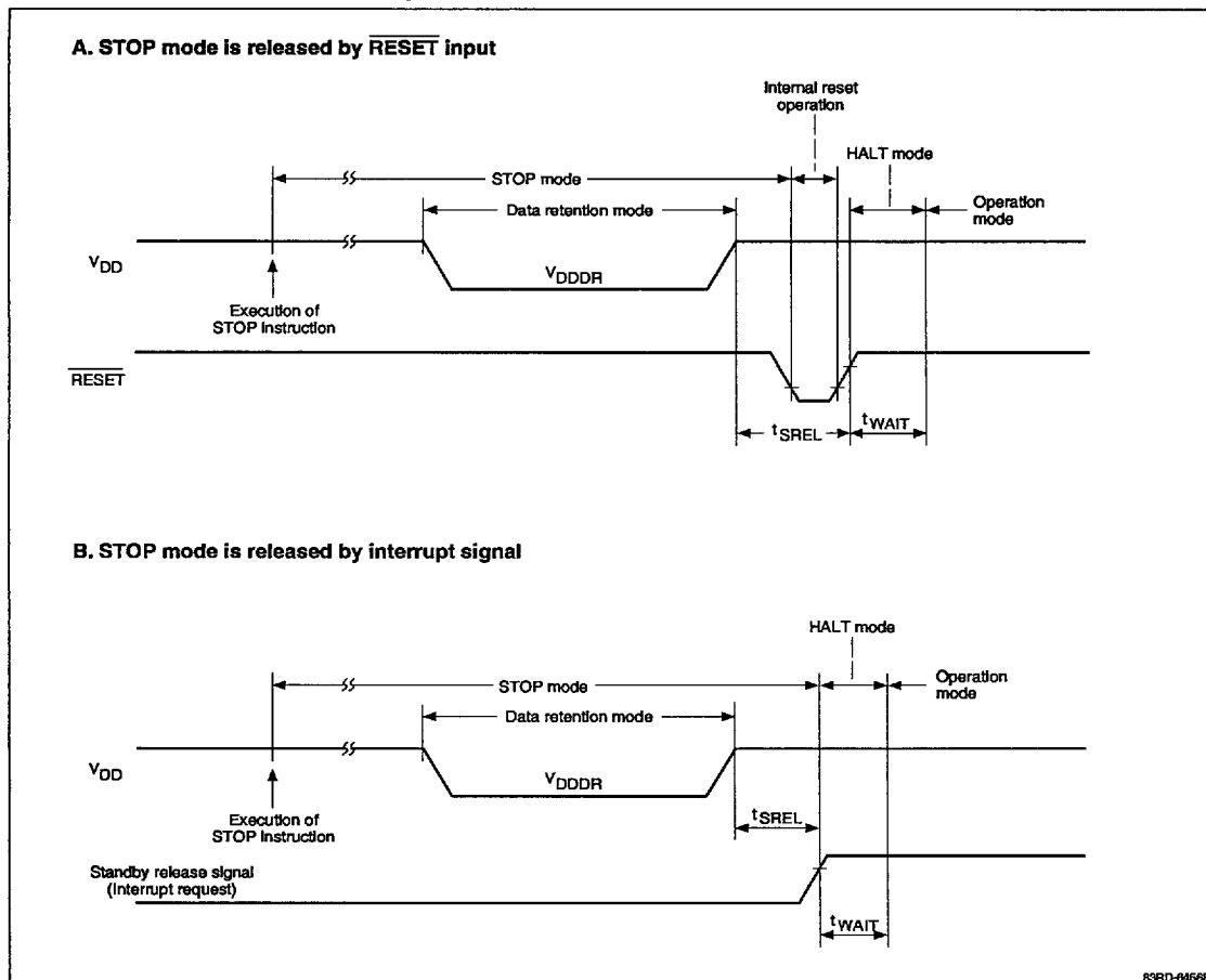
Figure 11. Data Retention Timing
