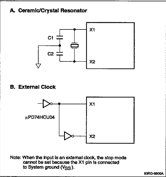
Figure 1. System Clock Configurations
