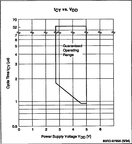
Figure 3. Main System Clock Operation; t CY vs V DD
