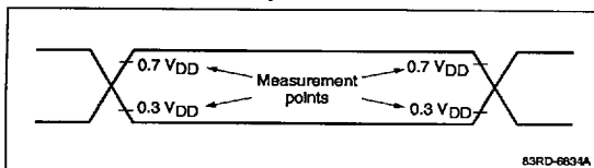
Figure 5. Clock Timing Measurement Points
