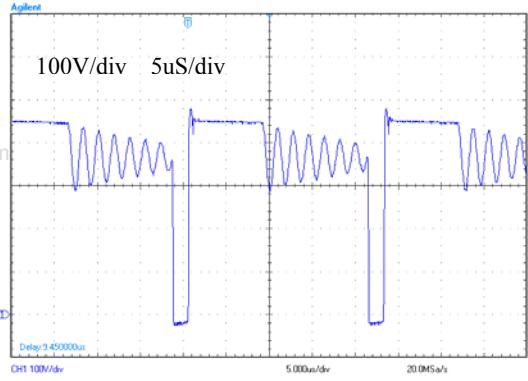
Vin=265V, Io=0.5A
