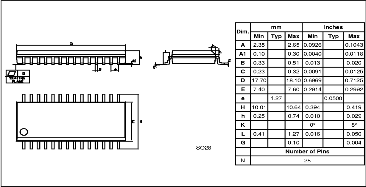
Figure 43. 28-Pin Plastic Small Outline Package, 300-mil Width
