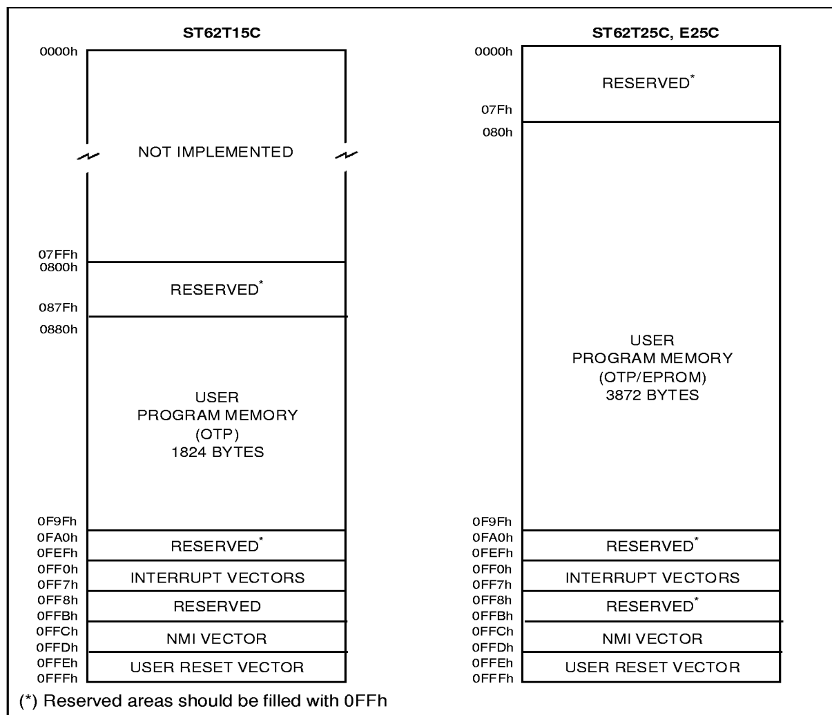
Figure 4. Program Memory Map
