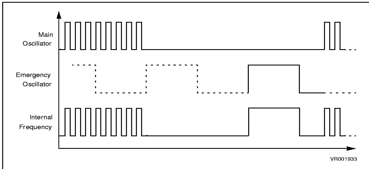
Figure 10. OSG Emergency Oscillator Principle
