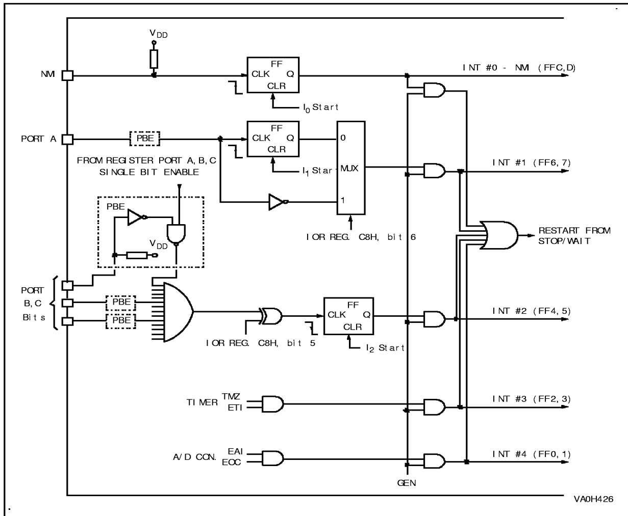
Figure 21. Interrupt Block Diagram
