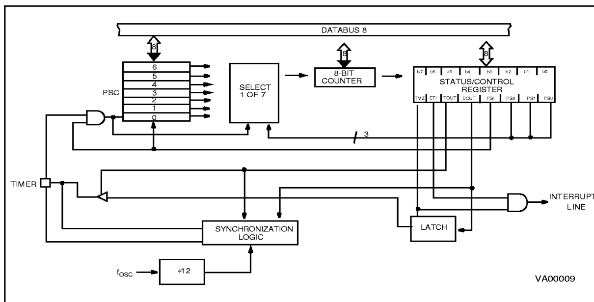
Figure 24. Timer Block Diagram
