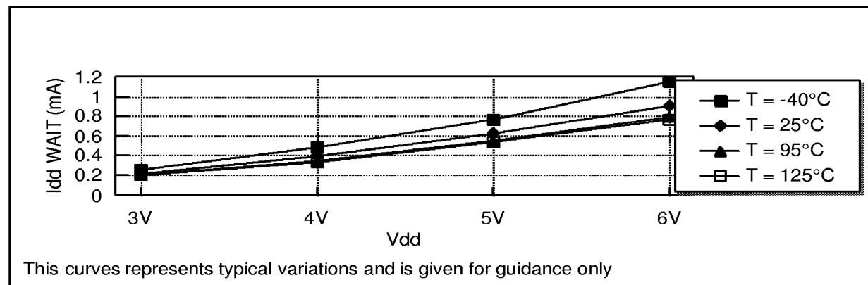
Figure 31. Idd STOP versus Vcc for OTP devices
