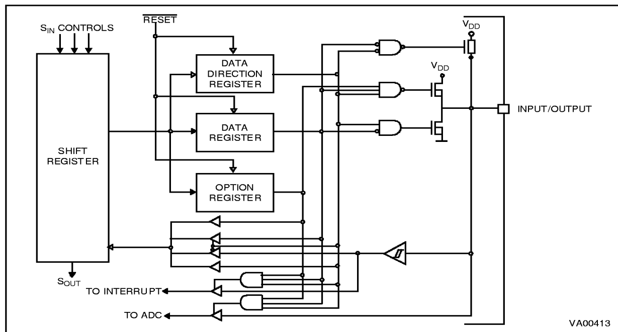
Figure 22. I/O Port Block Diagram
