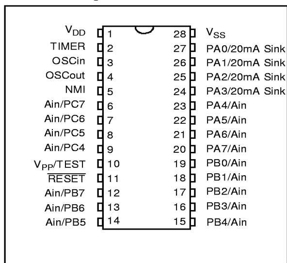
Figure 2. ST62T15C,T25C and E25C Pin Configuration
