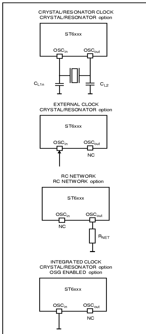
Figure 8. Oscillator Configurations
