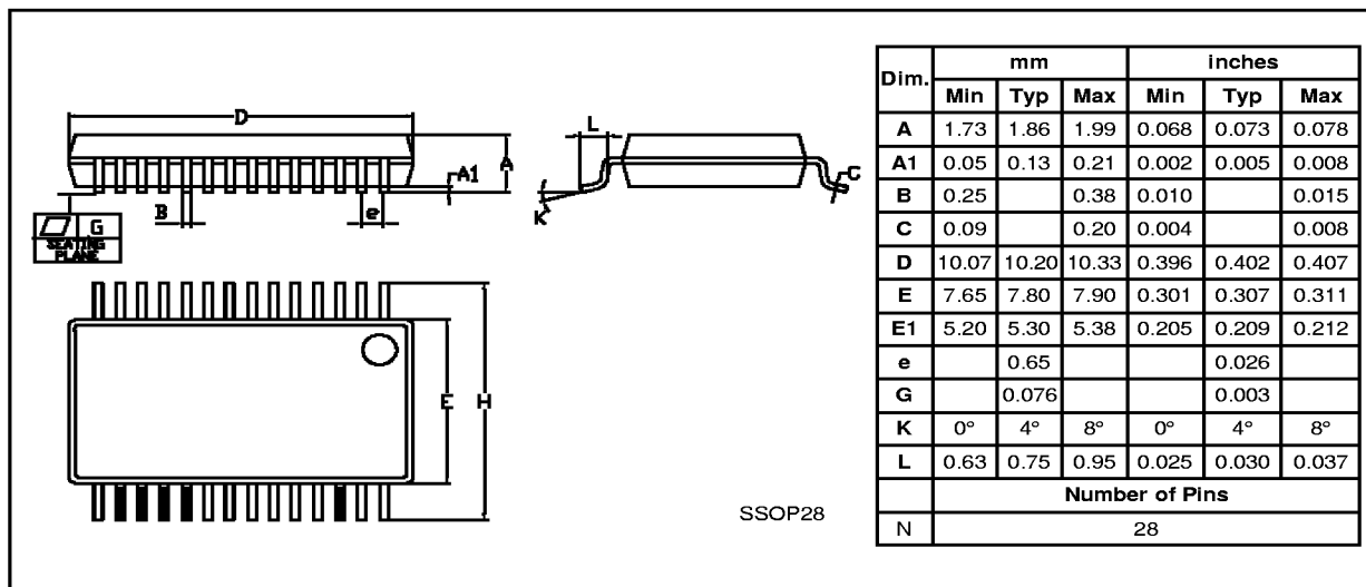
Figure 45. 28-Pin Plastic Shrink Small Outline Package, 0.209" Width
