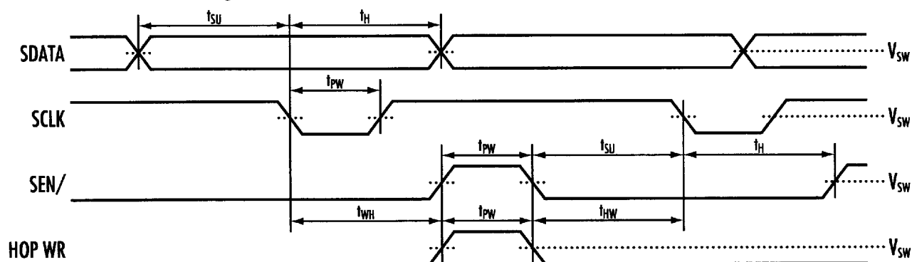
Figure 9. Serial Mode Interface AC Timing Waveforms
