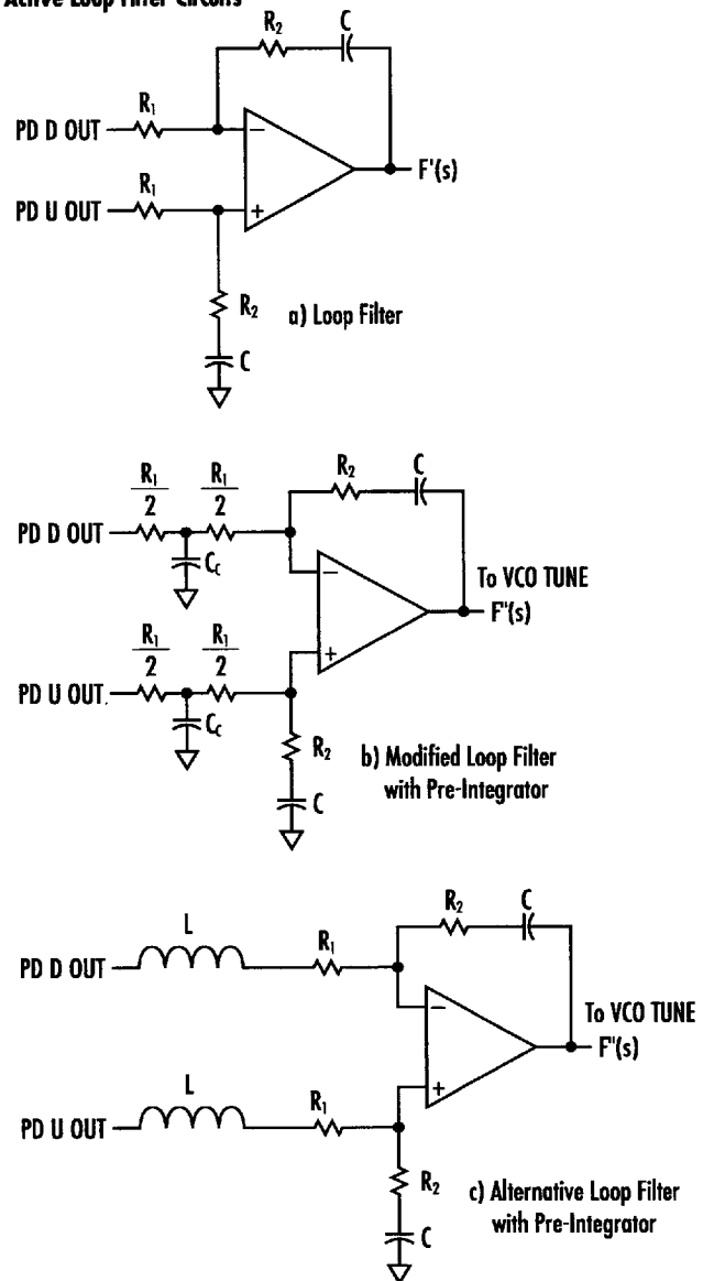
Figure 13. Active Loop Filter Circuits
