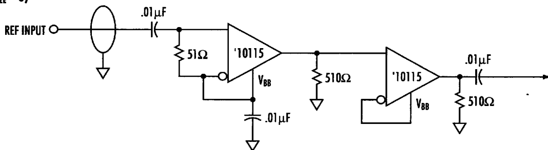
Figure 19. Optional Reference Input Line Receiver Circuit ( V_{CC} = +5 V, V_{EE} = 0 )
