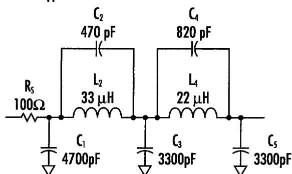
Figure 14. Reference Suppression Filter
