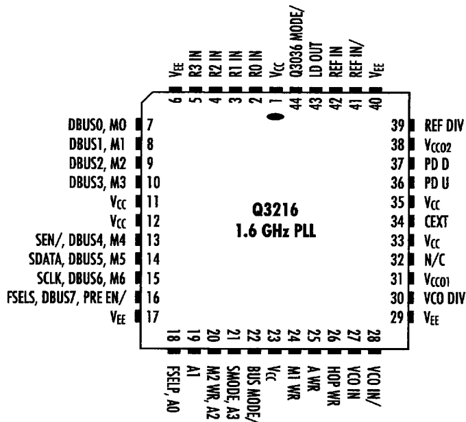
Figure 10. Q3216 44-pin Configuration
