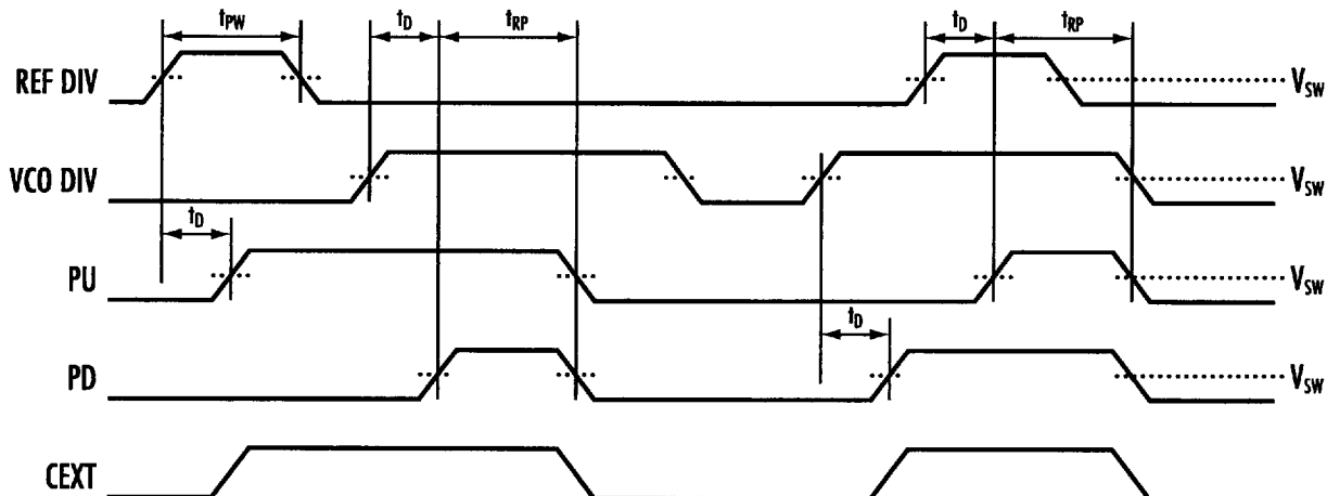
Figure 6. Phase/Frequency Detector Waveforms
