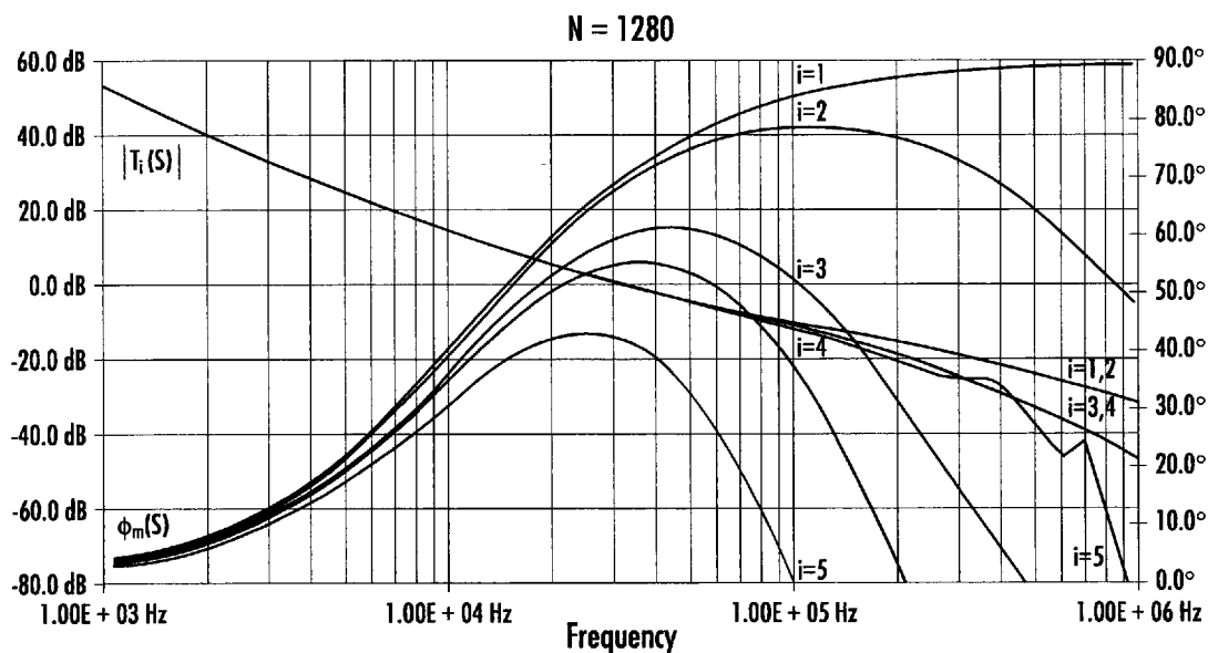
Figure 17. Bode Analysis - Open Loop Gain and Phase Margin
