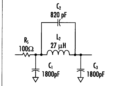
Figure 16. 1 MHz 3-pole Reference Suppression Filter
