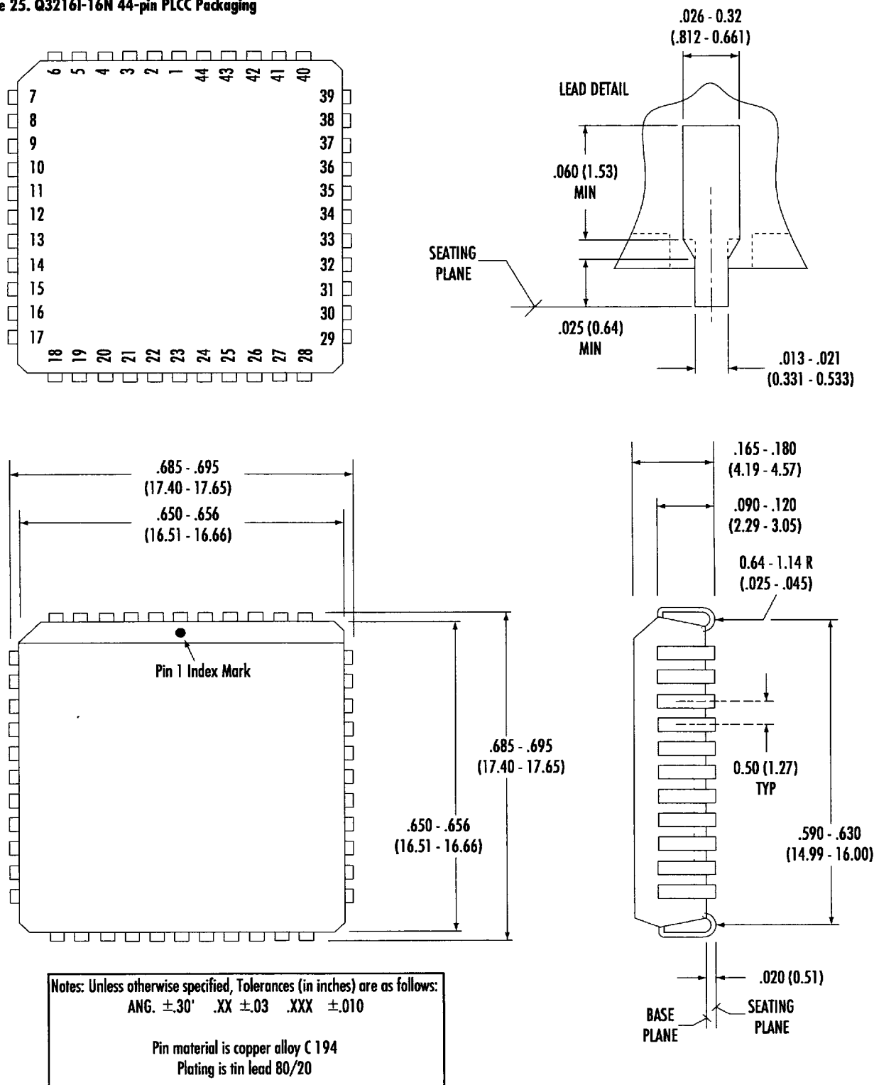
Figure 25. Q3216I-16N 44-pin PLCC Packaging
