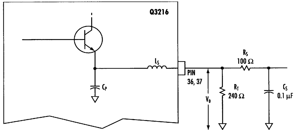
Figure 21. PD D, PD U Output Maximum Loading
