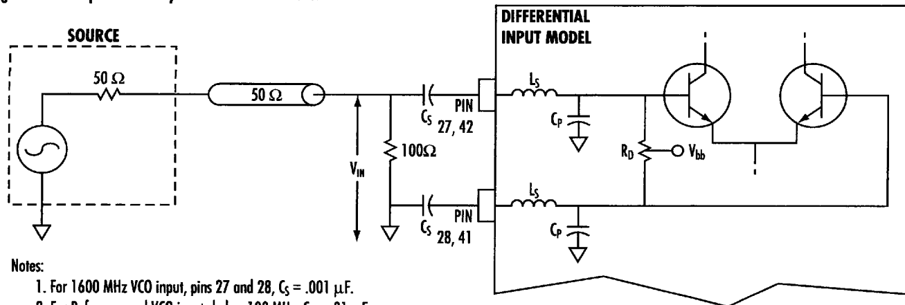
Figure 5. VCO Input Sensitivity Measurement Test Circuit
