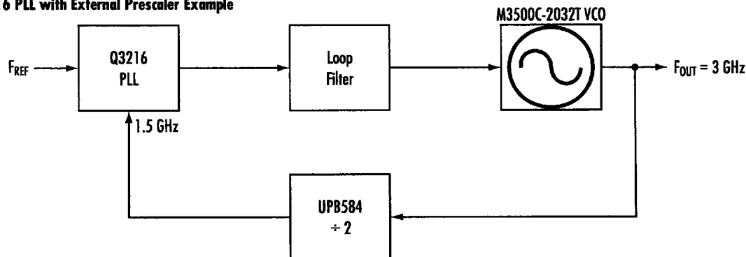
Figure 23. Q3216 PLL with External Prescaler Example
