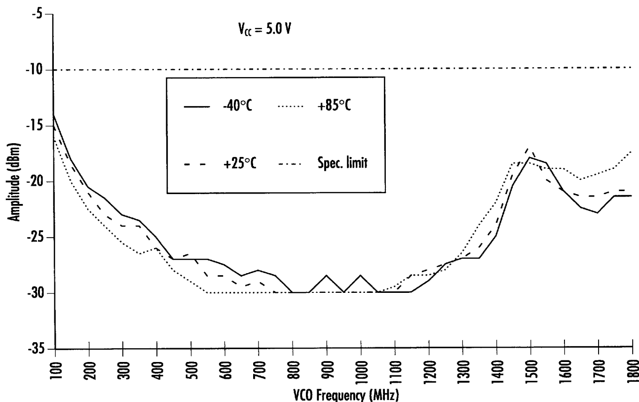
Figure 4. VCO Sinusoidal Input Sensitivity
