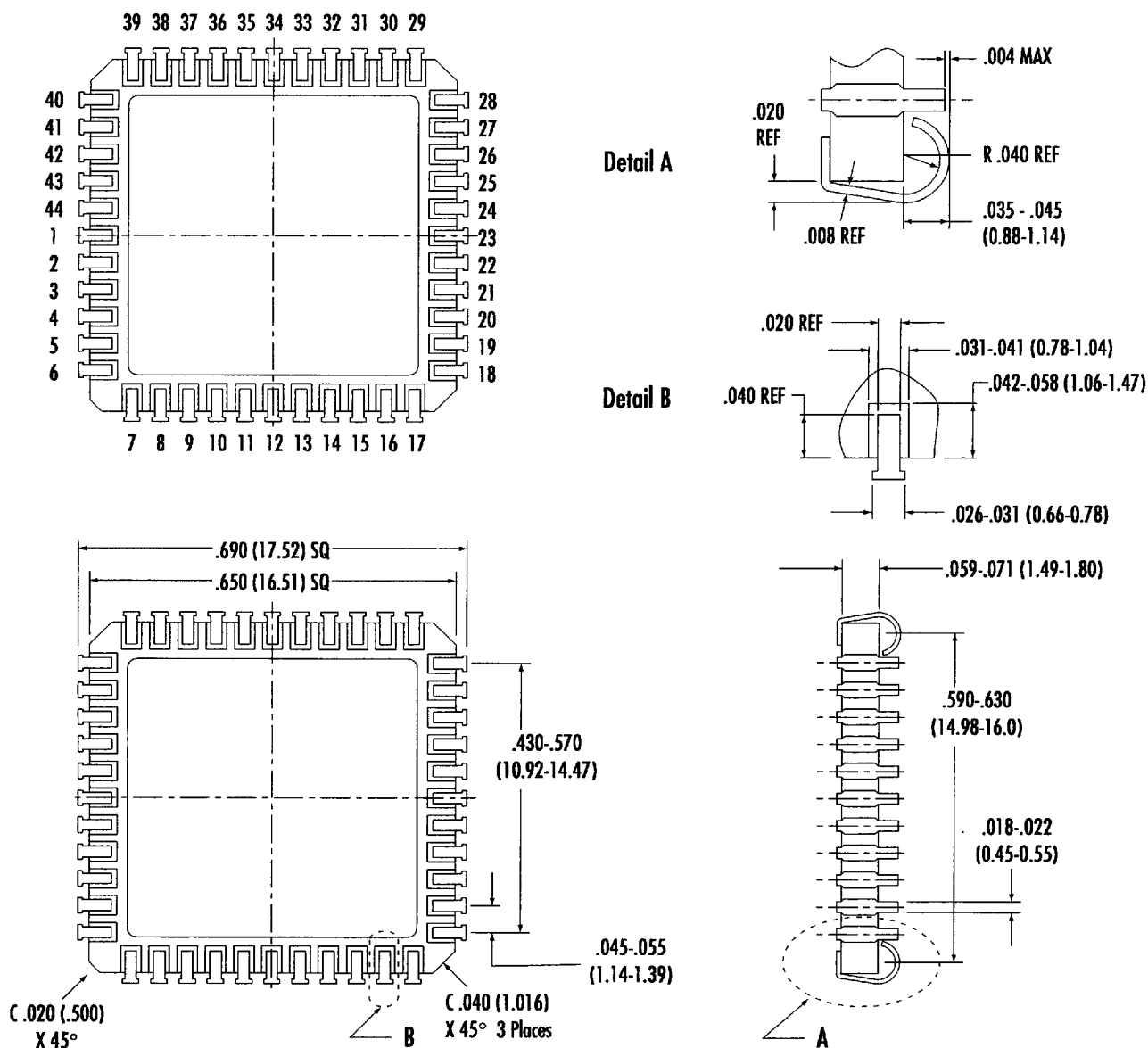
Figure 26. Q3216M-16L 44-pin CLDCC Packaging
