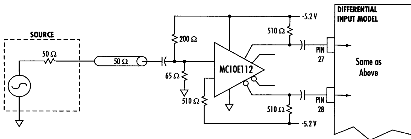
b) Differential (balanced) Input
