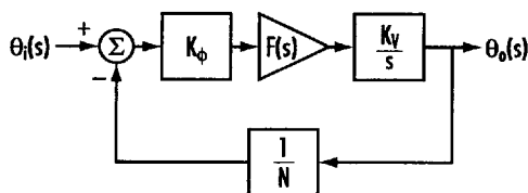
Figure 12. Second Order Type II PLL
