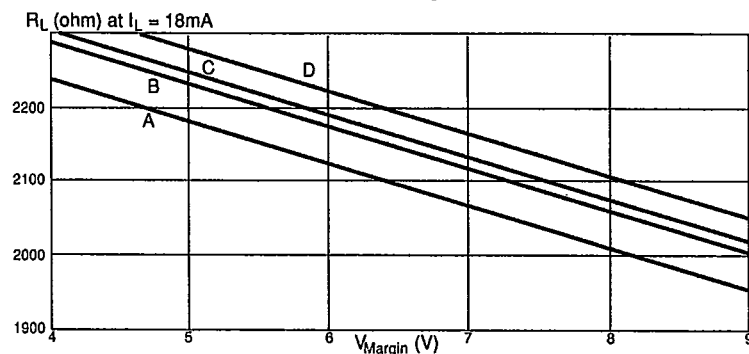
Figure 17. Loop resistance at I_L = 18\text{mA} as a function of V_{Margin} at open loop.
