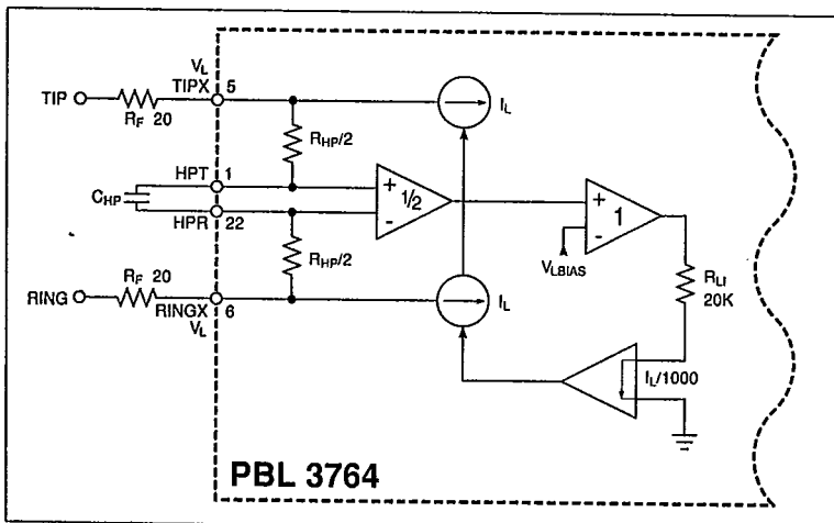
Figure 9. Longitudinal impedance.
