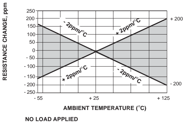
FIGURE 3 - TEMPERATURE COEFFICIENT RESISTANCE
