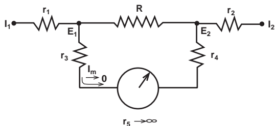
FIGURE 5 - KELVIN CONNECTION
