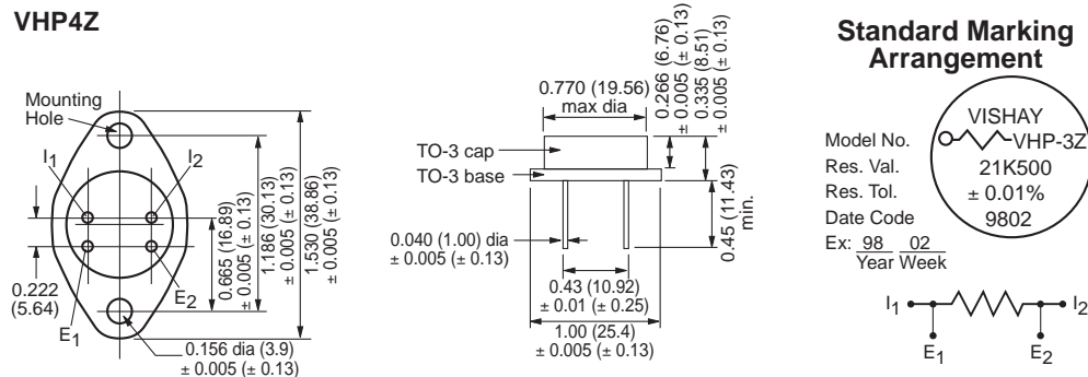
FIGURE 6 - STANDARD IMPRINTING AND DIMENSIONS
