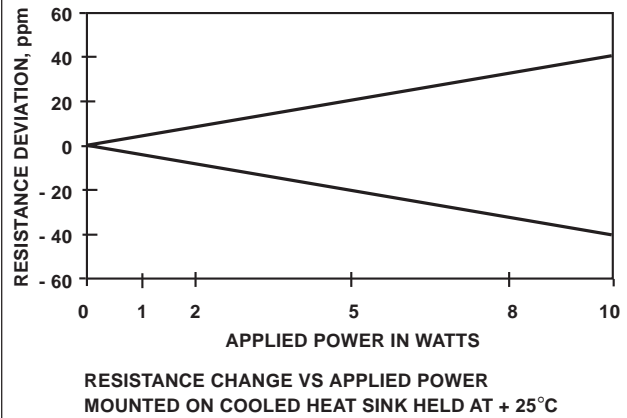
FIGURE 2 - POWER COEFFICIENT (WCR)
