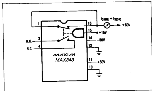
Figure 8. ON Leakage Test Circuit.
