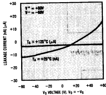
OFF LEAKAGE vs. SWITCH VOLTAGE
