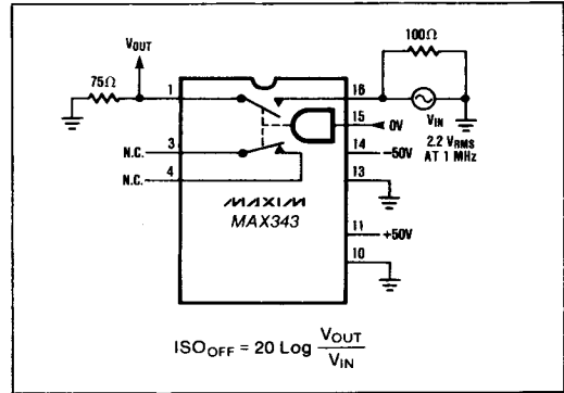
Figure 4. OFF Isolation Test Circuit.
