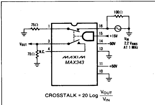
Figure 5. Channel-Channel Crosstalk Test Circuit.
