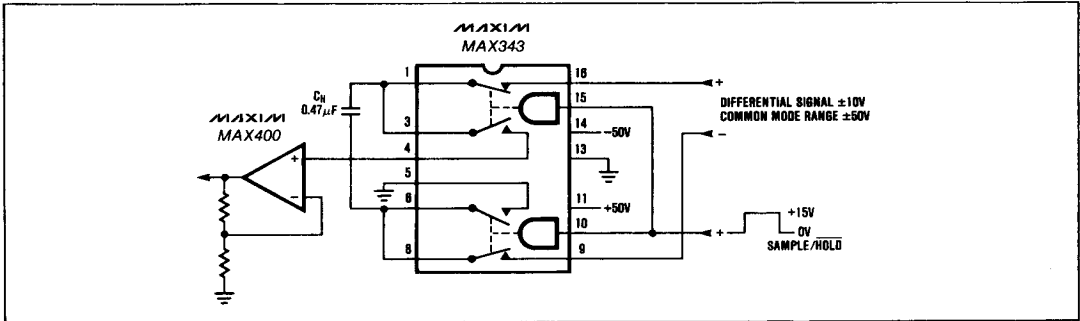
Figure 2. Flying Capacitor Differential to Single-Ended Converter with \pm 50V Common-Mode Range.
