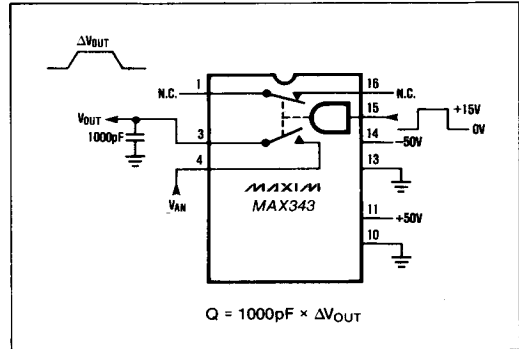
Figure 6. Charge Injection Test Circuit.
