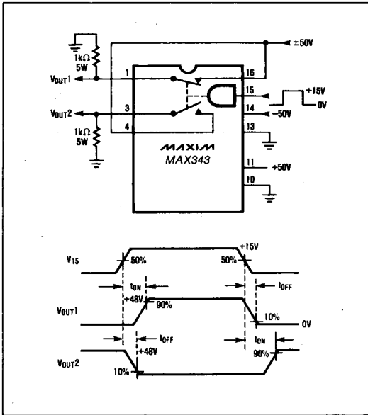
Figure 9. Switching Time Test Circuit.
