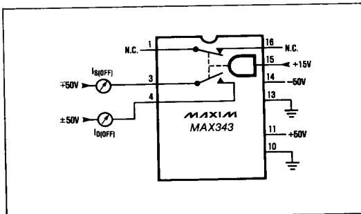
Figure 7. OFF Leakage Test Circuit.
