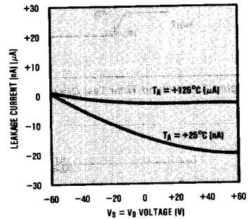
ON LEAKAGE vs. SWITCH VOLTAGE
