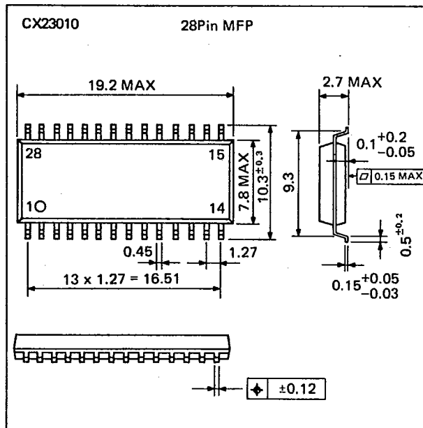
Package outline
