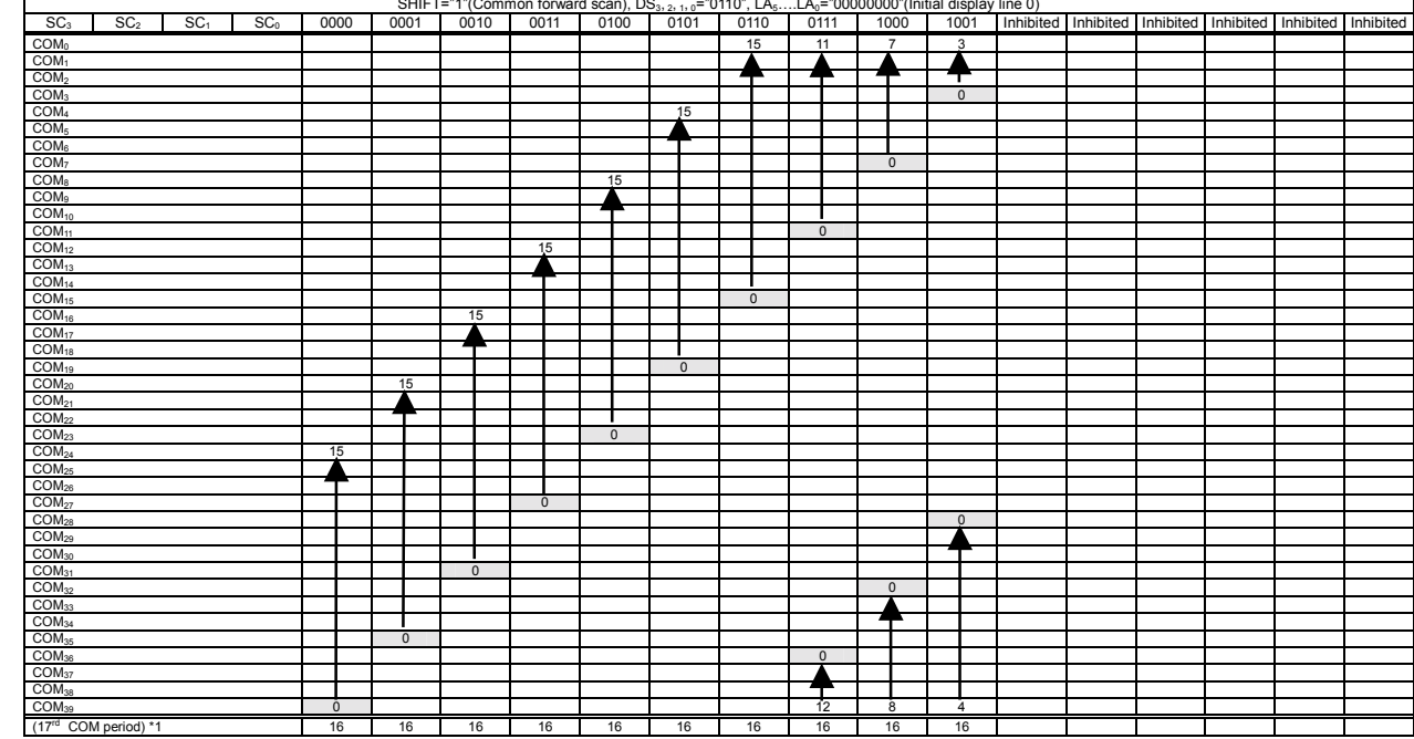
(32-4) Initial display line “0”, 1/17 duty cycle (Common backward scan, DSE=“0”)
