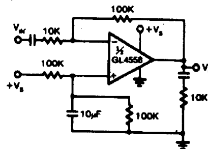
AC Coupled Inverting Amplifier
