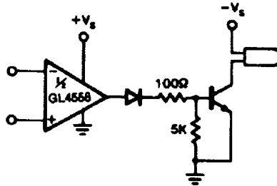
Lamp Driver
