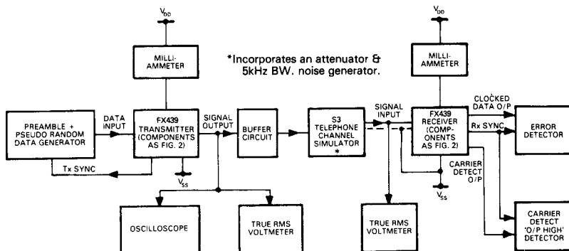
Fig. 4 FX439 Test set-up.
