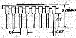
16 LEAD CERAMIC DUAL-IN-LINE
