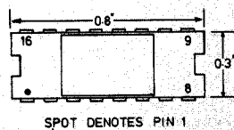
FIG.15 PACKAGE DETAIL
