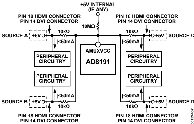
Figure 28. Suggested AMUXVCC Power Scheme
