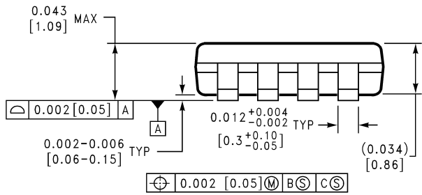
NS Package Number MUA008AE
