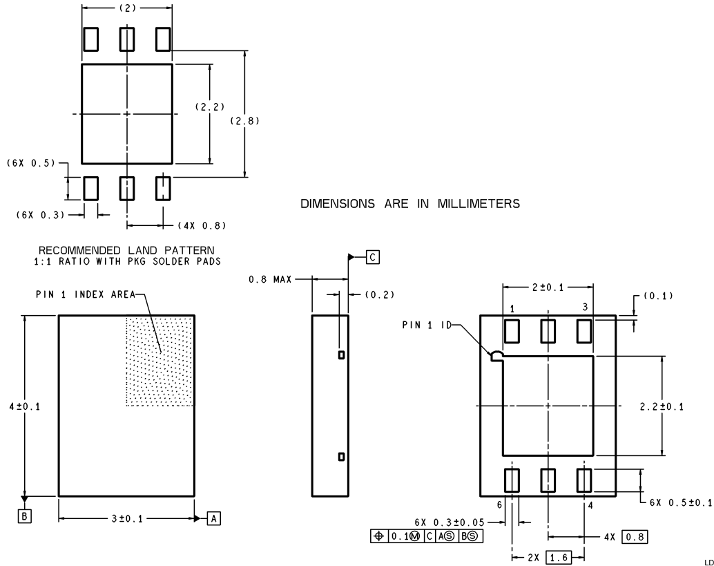
NS Package Number LDC06D
