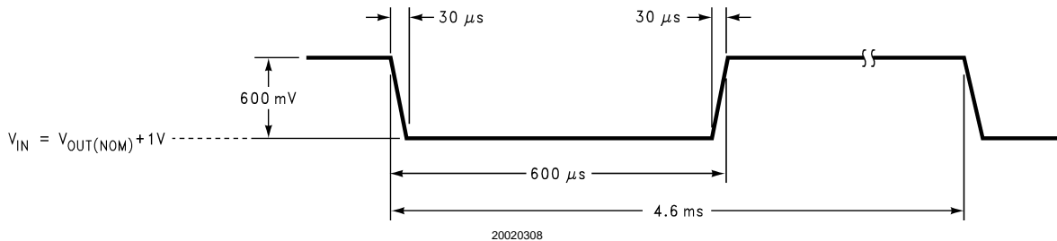
FIGURE 1. Line Transient Response Input Perturbation
