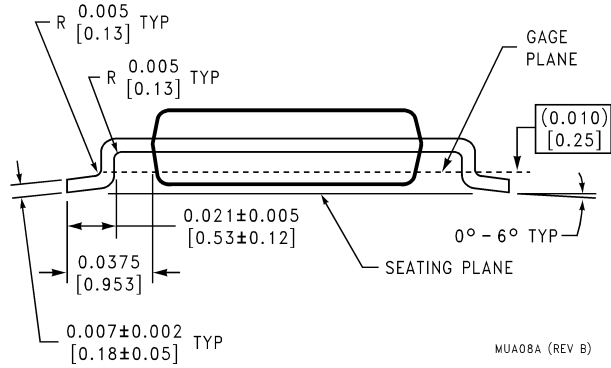
NS Package Number MUA008AE
