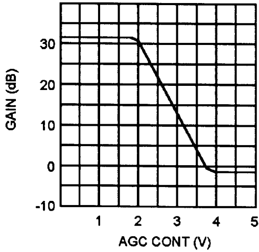
Fig.3A - \gamma 1 I/O characteristics
