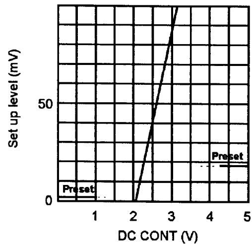
Fig.5 - Dark clip control characteristics
