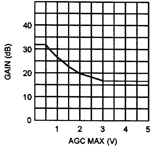
Fig.3B - \gamma 2 I/O characteristics
