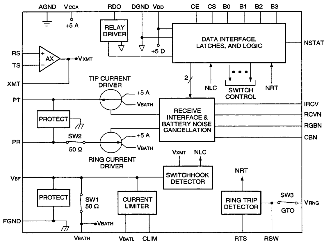
Figure 1. Architectural Diagram
