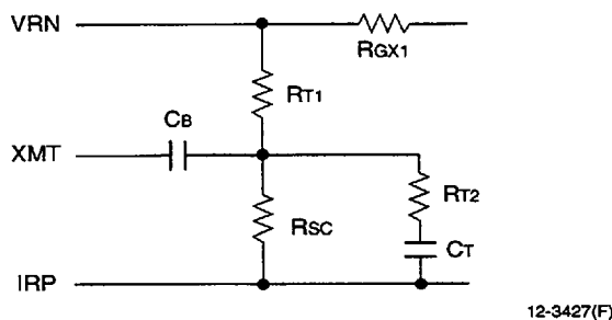
Figure 13. Addition of Resistor R_{SC} from XMT to IRP
