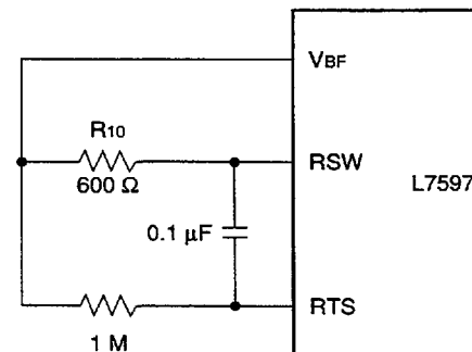
Figure 9. Ring Trip Threshold
