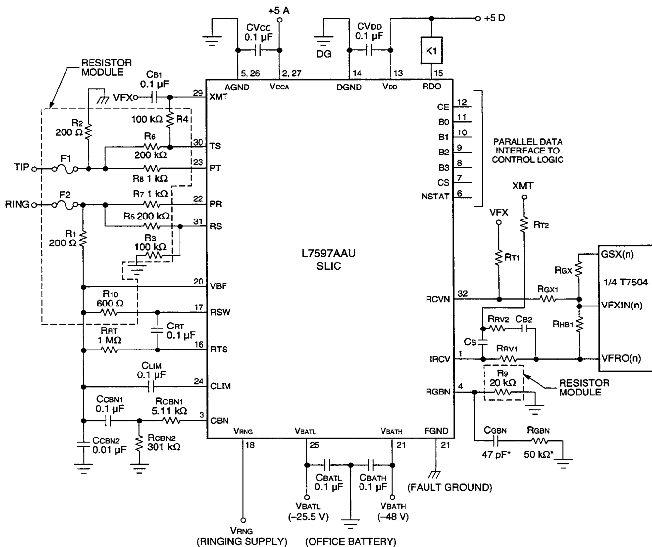
Figure 5. External Components Required
