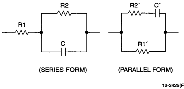
Figure 10. Equivalent Complex Terminations
