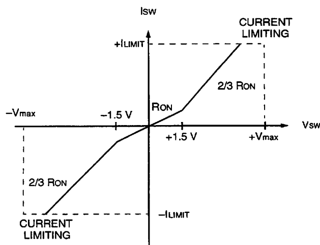
Figure 3. Switch On-State V-I Characteristics SW1 and SW2
