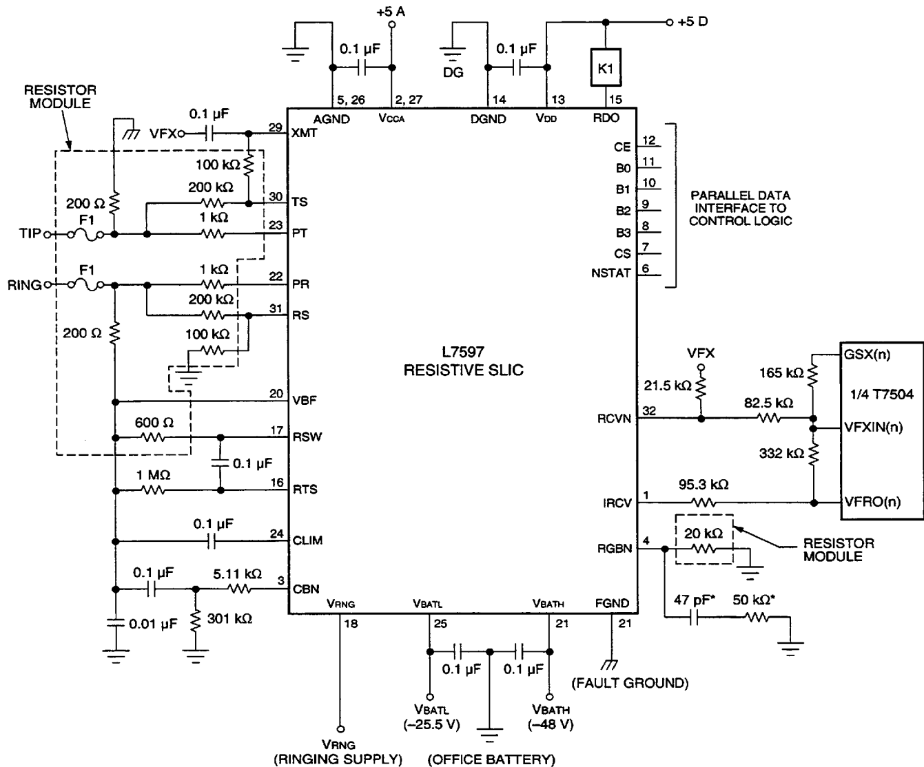
Figure 14. TA-909 Application Diagram
