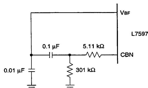
Figure 8. Implementing the Noise Cancellation Function
