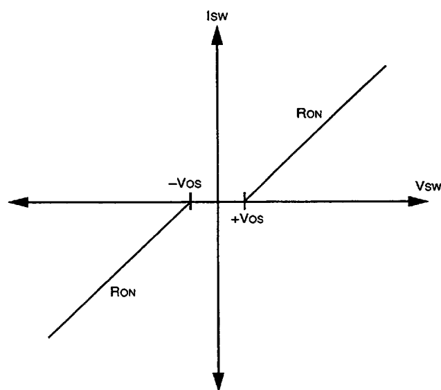
Figure 4. Switch On-State V-I Characteristics SW3
