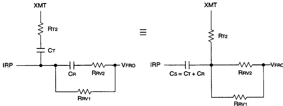
Figure 12. Revised ac Interface C_T and C_R Combined into a Single Capacitor C_S
