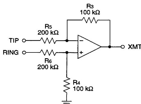
Figure 7. L7597 SLIC Matching Requirements
