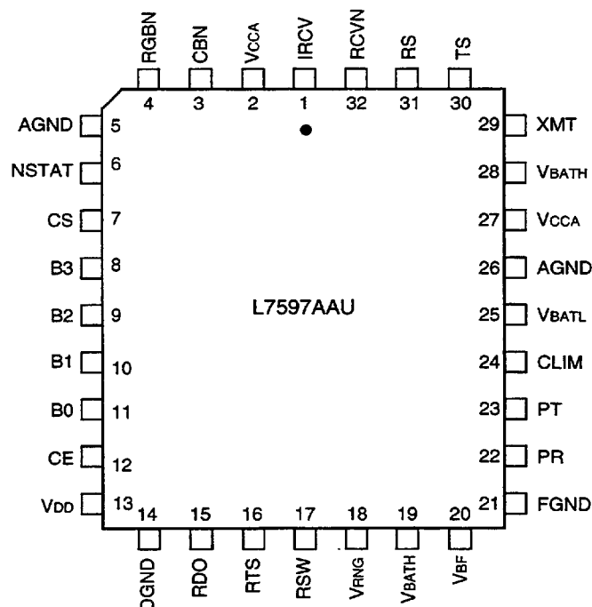
Figure 2. Pin Layout
