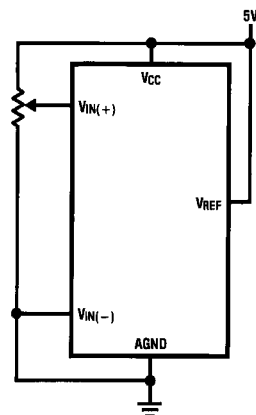
FIGURE 3. Ratiometric
