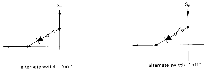
Fig. 4 Alternate Switch
