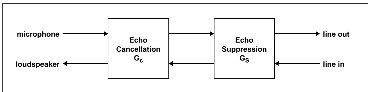
Figure 11 Speakerphone - Block Diagram
