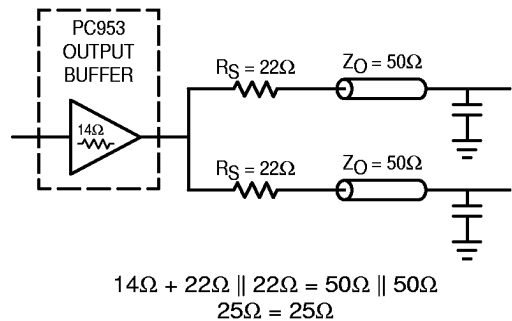
Figure 6. Optimized Dual Line Termination
