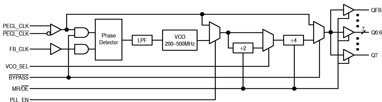
Figure 1. Logic Diagram
