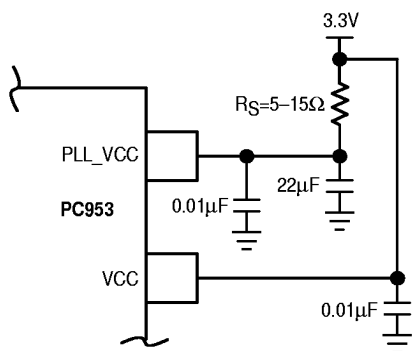
Figure 3. Power Supply Filter
