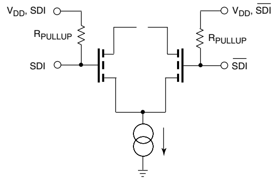
Fig. 4 Serial Data &amp; Clock Input Circuit
