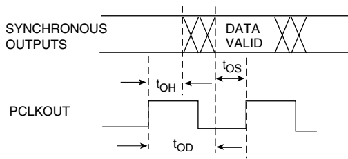
Fig. 3 Output Delay &amp; Hold Times (Synchronous Outputs)
