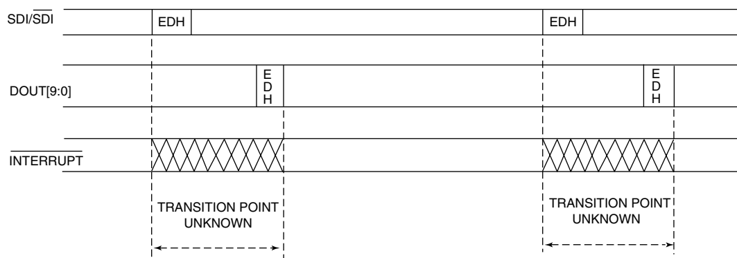
Fig. 11 \overline{\text{INTERRUPT}} Timing
