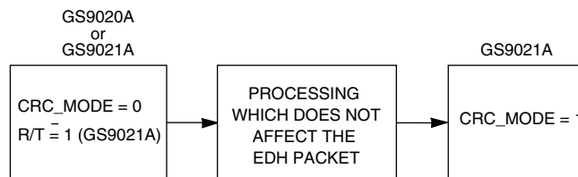
Fig. 13a Example of CRC_MODE Implementation
