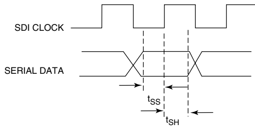
Fig. 1 Serial Data Input Setup &amp; Hold Times
