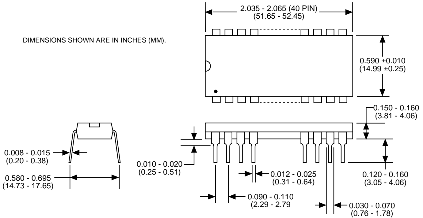
FIGURE 15. RDC-19220S (40-PIN DDIP) PLASTIC PACKAGE MECHANICAL OUTLINE
