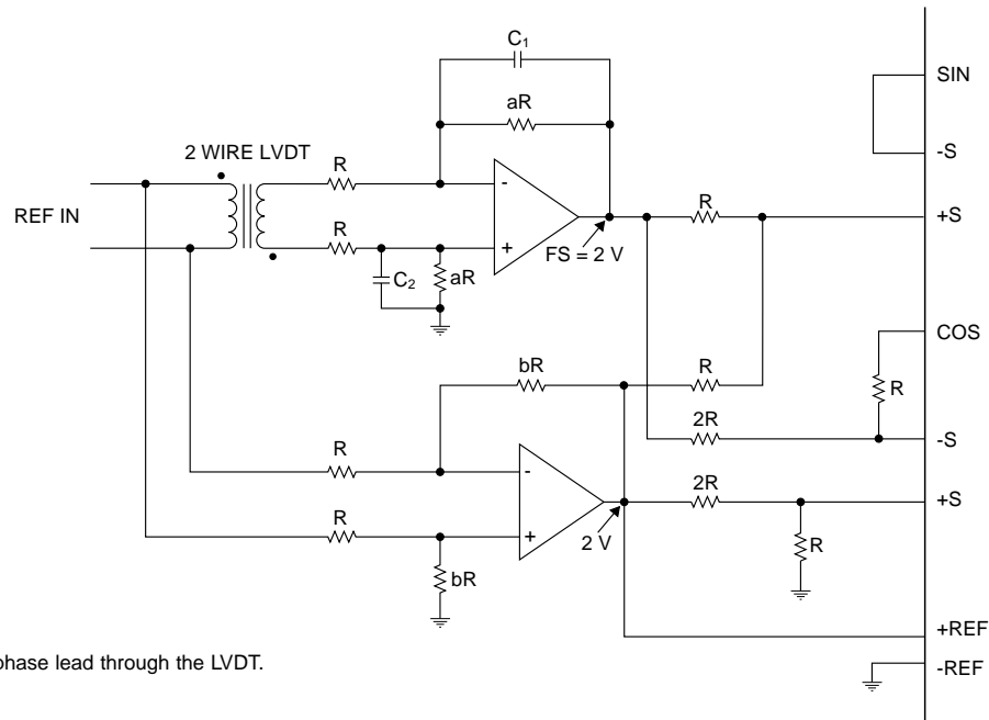
FIGURE 11A. 2-WIRE LVDT DIRECT INPUT
