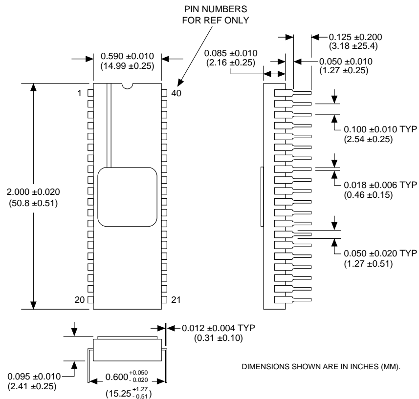
FIGURE 16. RDC-19220S (40-PIN DDIP) CERAMIC PACKAGE MECHANICAL OUTLINE
