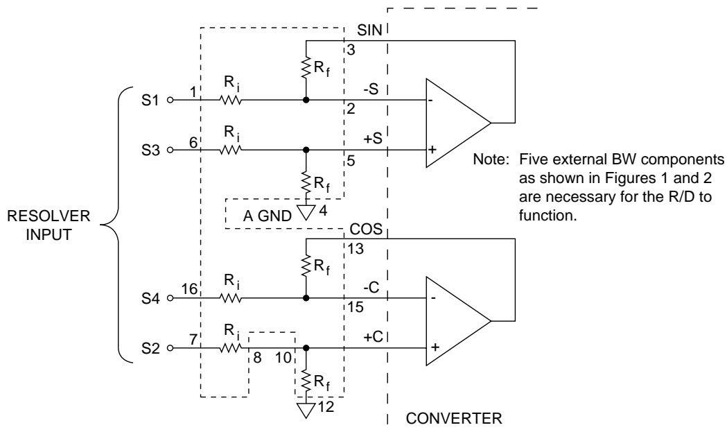
FIGURE 9A. DIFFERENTIAL RESOLVER INPUT
