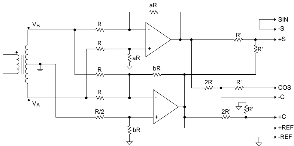
FIGURE 11A. 2-WIRE LVDT DIRECT INPUT
