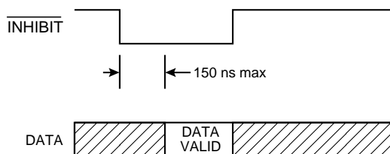
FIGURE 12. INHIBIT TIMING
