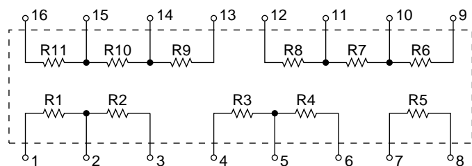
FIGURE 20. (DDC-49530, DDC-49590, DDC-57470) LAYOUT AND RESISTOR VALUES (SEE TABLE 9)
