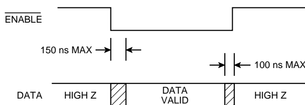
FIGURE 13. ENABLE TIMING
