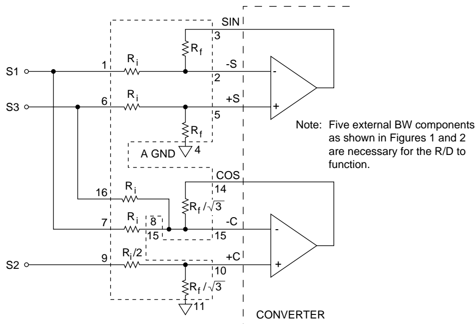
FIGURE 9C. SYNCHRO INPUT
