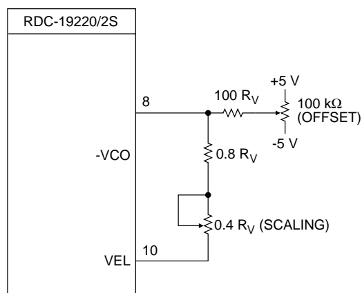
FIGURE 10. VELOCITY TRIMMING
