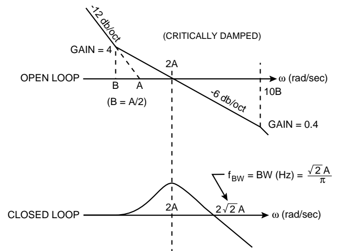
FIGURE 4. BODE PLOTS
