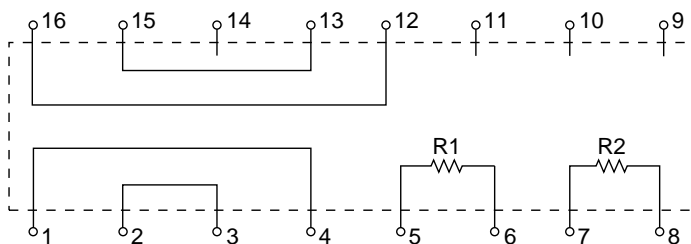
FIGURE 19. (DDC-55688-1) LAYOUT AND RESISTOR VALUES (R1 AND R2 = 10 K \Omega 1.0% TOL, ABSOLUTE TC = \pm 100 PPM MAX)
