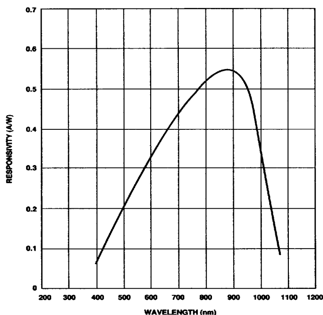
Fig.13 SERIES 0 - TYPICAL SPECTRAL RESPONSE
