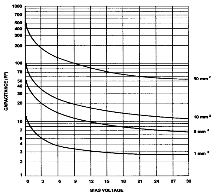
Fig.14 SERIES 0 - TYPICAL CAPACITANCE VERSUS BIAS VOLTAGE FOR A GIVEN DETECTOR AREA
