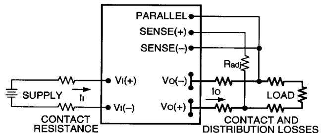
Figure 6. Circuit Configuration to Adjust Output Voltage
