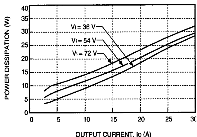
Figure 10. Power Dissipation as Heat vs. Output Current
