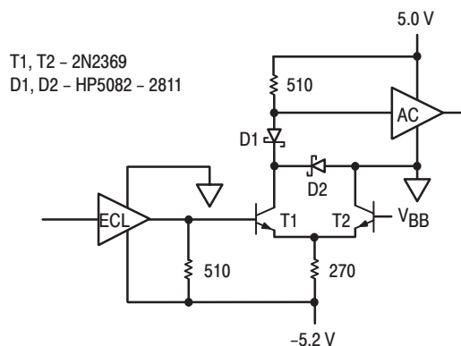
Figure 1-36b. Single-Ended ECL-to-'AC Circuit
