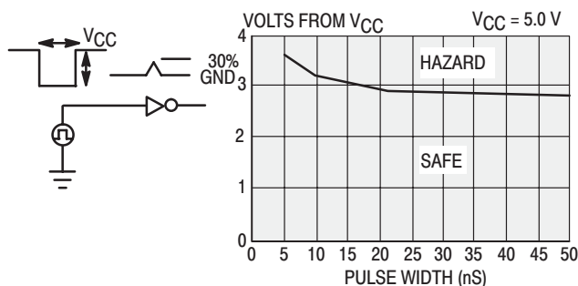
Figure 1-42a. High Noise Margin
