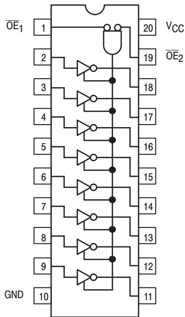
Figure 1. MC74AC540/74ACT540
