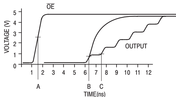
Figure 1-56. Measurement Stepout
