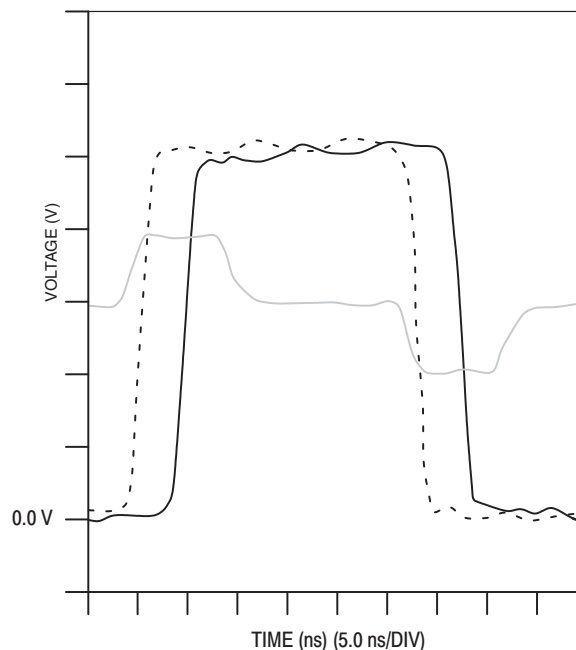
Figure 1-41b. Reverse Crosstalk on PCB Traces
