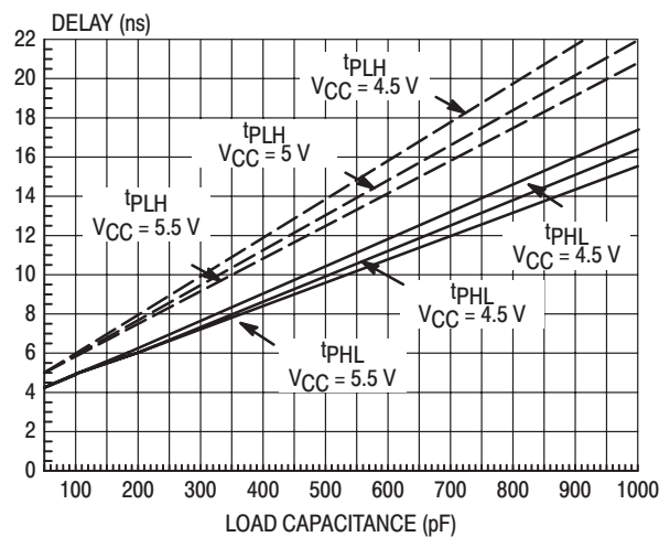
Figure 1–13. Propagation Delay versus C_L ('AC00)
