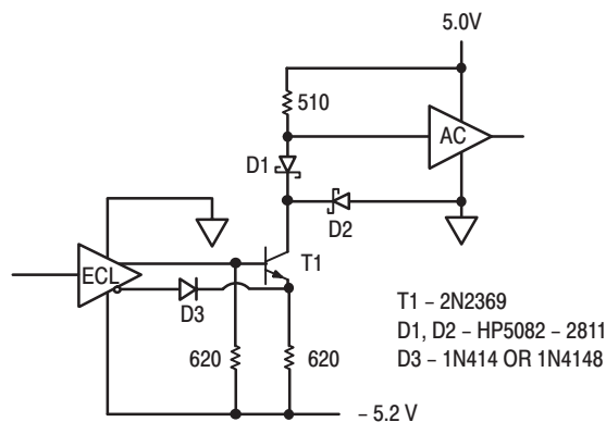
Figure 1-36c. Differential Output ECL-to-'AC Circuit
