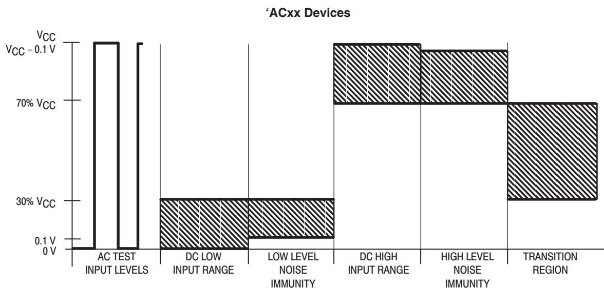
Figure 1-22a. Test Input Signal Levels
