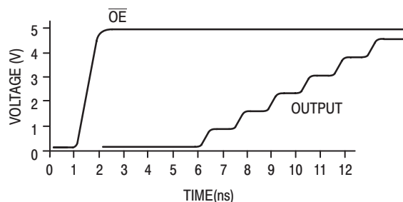
Figure 1-55. Typical ATE 3-State Waveform
