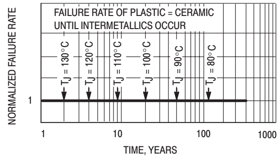
Figure 1–32. Failure Rate versus Time Junction Temperature
