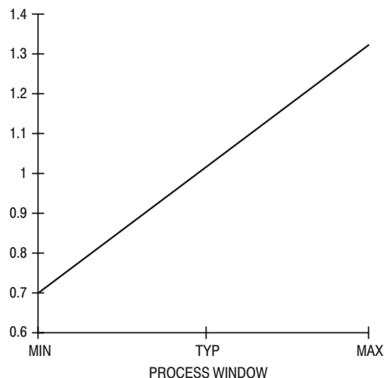
Figure 1-11d. FACT Process Effects on Delay Times
