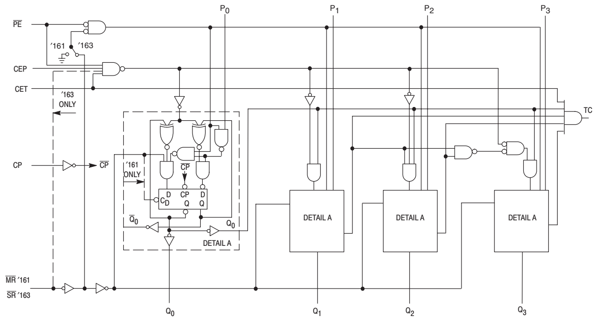
Figure 4. Logic Diagram
