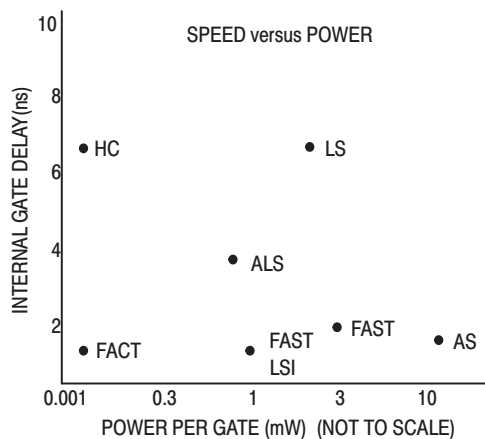
Figure 1-7. Internal Gate Delays
