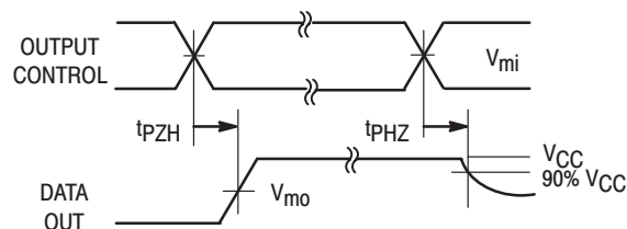
Figure 1–26. 3-State Output High Enable and Disable Times
