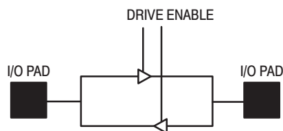
Figure 1-51. '245 I/O Structure
