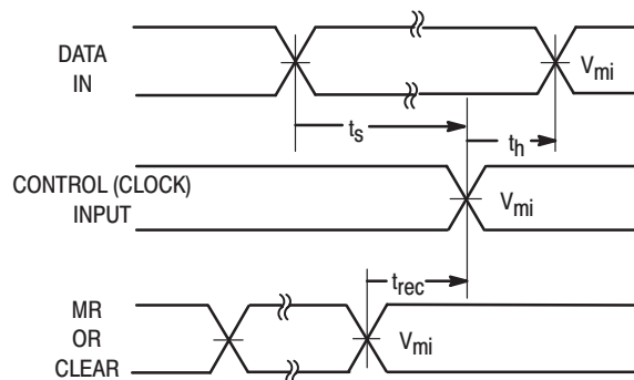
Figure 1–25. Setup Time, Hold Time and Recovery Time
