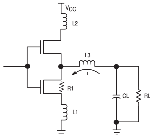
Figure 1-44a. Output Model
