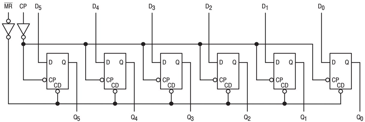
Figure 3. Logic Diagram
