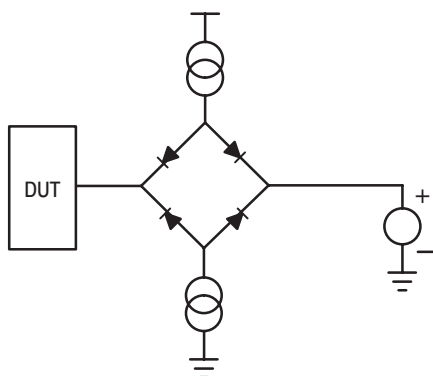
Figure 1-54. MCT Wheatstone Bridge Test Load
