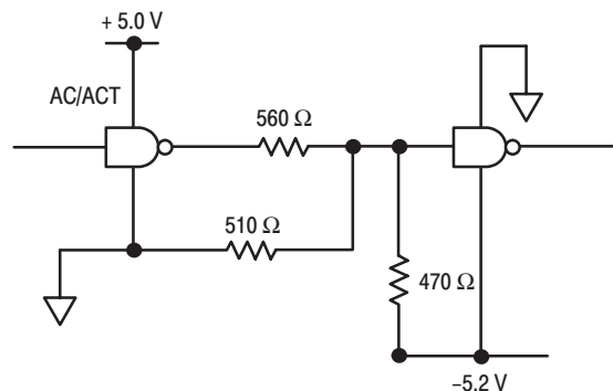
Figure 1-36a. Resistive FACT-to-ECL Translation
