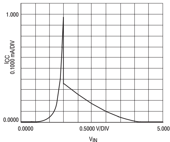
Figure 1–49. I_{CC} versus Input Voltage for 'ACT Devices
