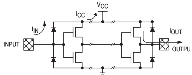
Figure 1–40. Noise Effects
