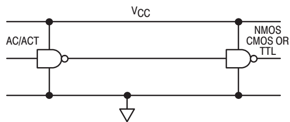
Figure 1-33. Interfacing FACT to NMOS, CMOS and TTL
