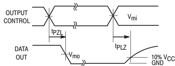
Figure 1–27. 3-State Output Low Enable and Disable Times
