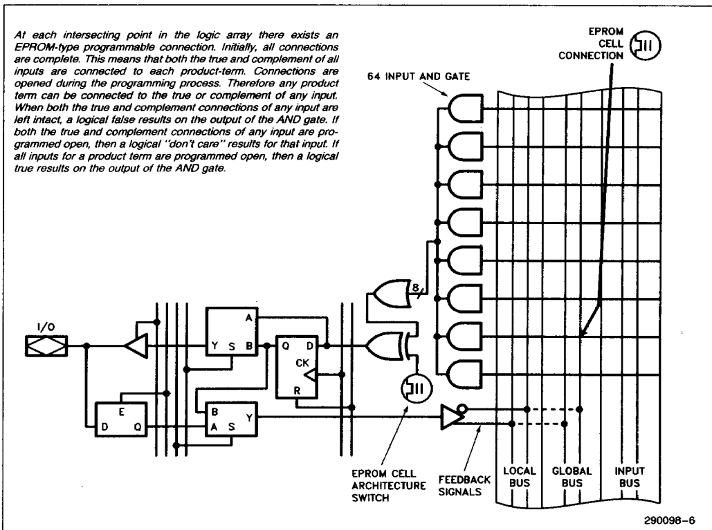
Figure 4. Macrocell-Bus Interface
