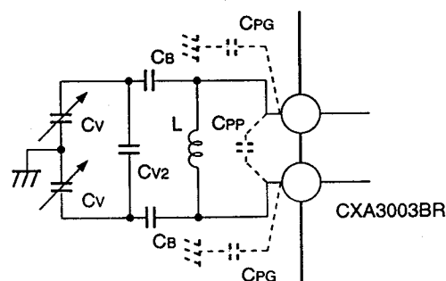
Fig. 13 VCO capacitors
