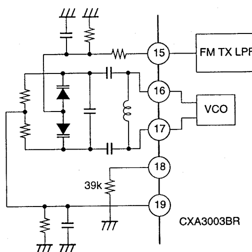
Fig. 12 Transmit VCO
