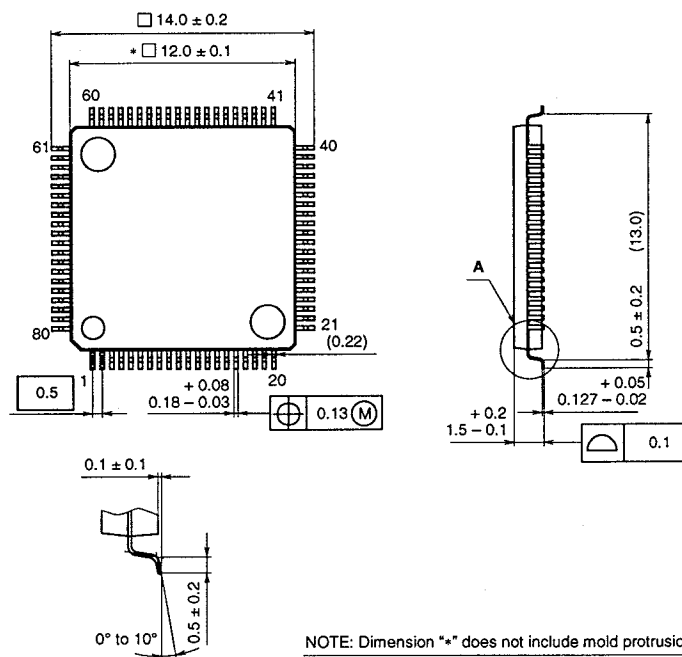
DETAIL A
