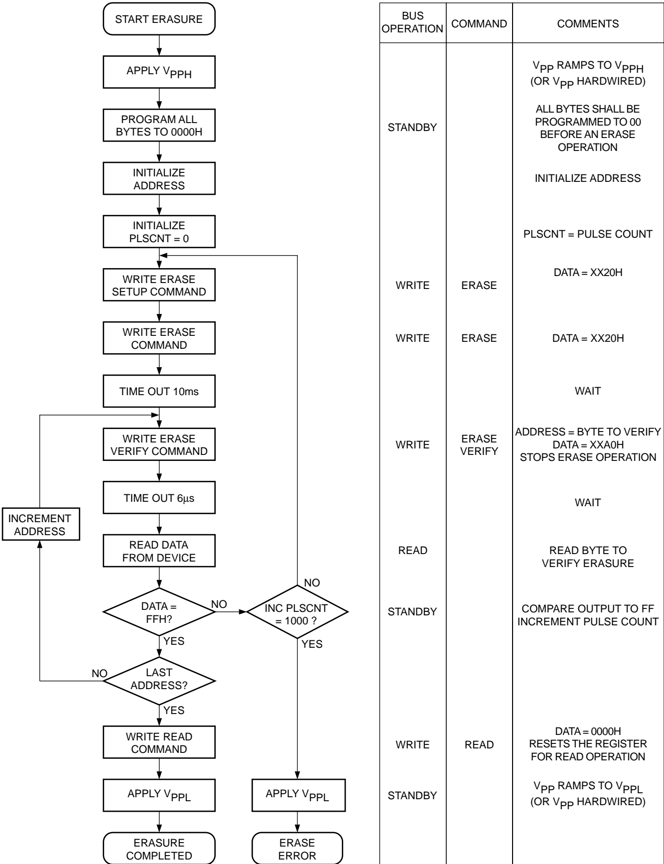
Figure 7. Chip Erase Algorithm (1)
