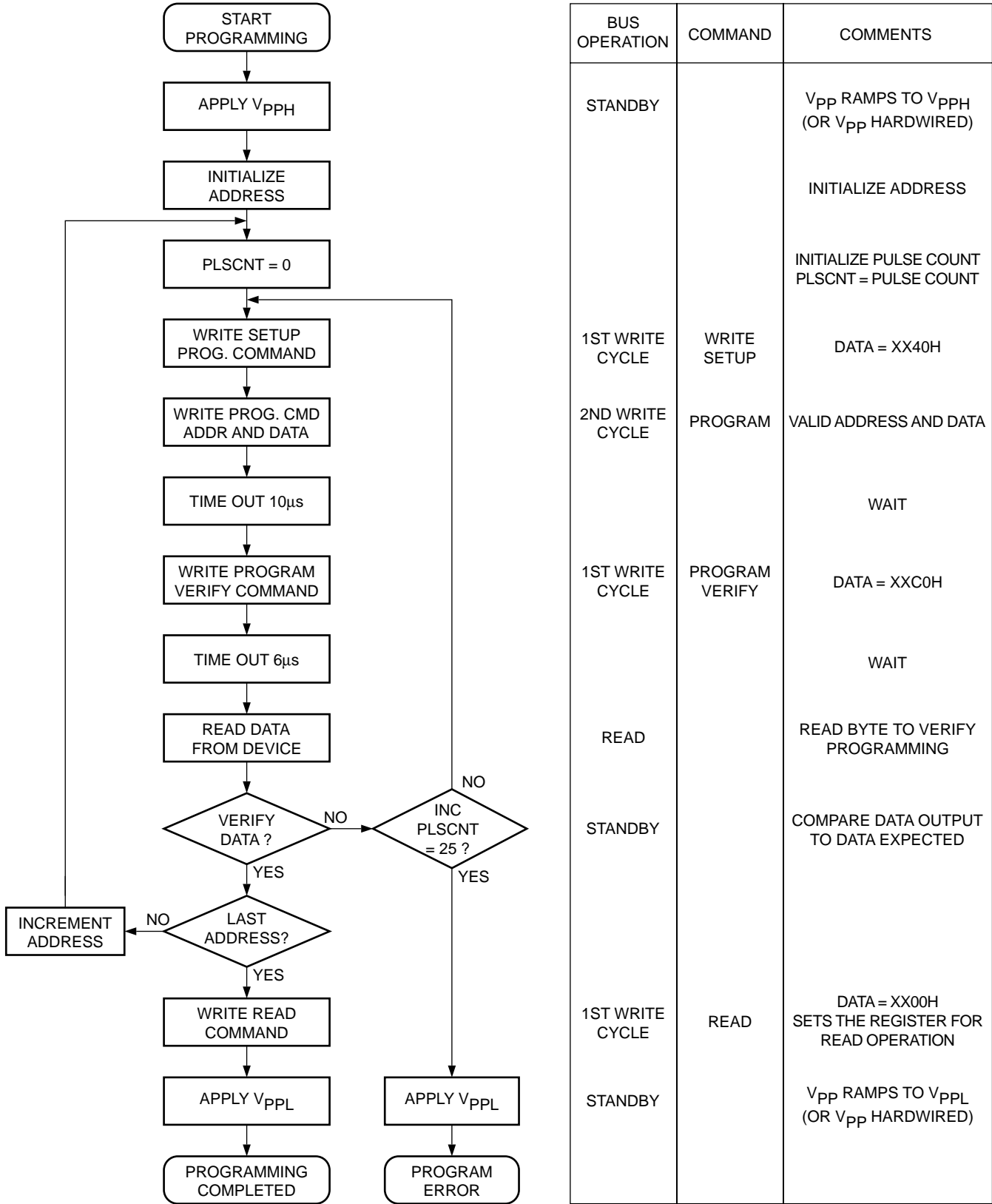
Figure 9. Programming Algorithm (1)
