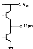
Figure 11 Speed discriminator (pin 11)
