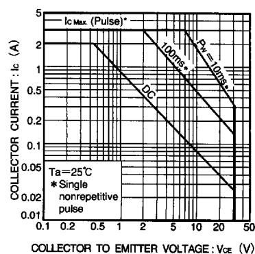
Fig.12 Safe operating area (2SD1055, 2SD1919)
