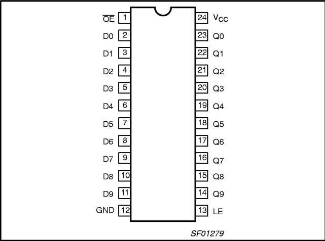
PIN CONFIGURATION for 74F841
