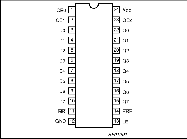
PIN CONFIGURATION for 74F845
