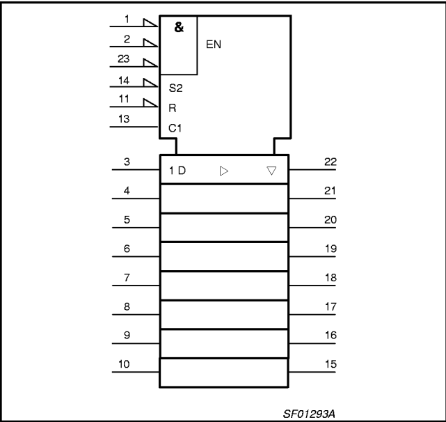
LOGIC SYMBOL (IEEE/IEC) for 74F845
