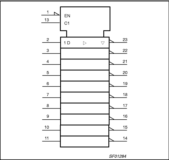
LOGIC SYMBOL (IEEE/IEC) for 74F842
