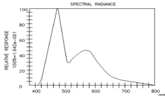
Luminous Spectrum (Ta=25°C)
