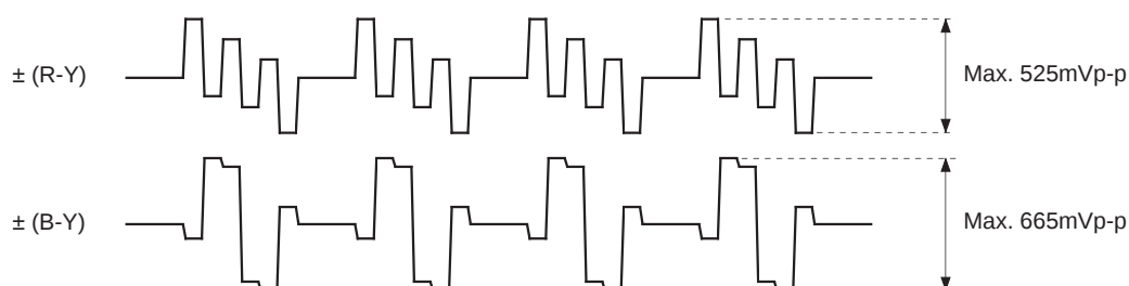
NTSC/PAL Signal (Example)
