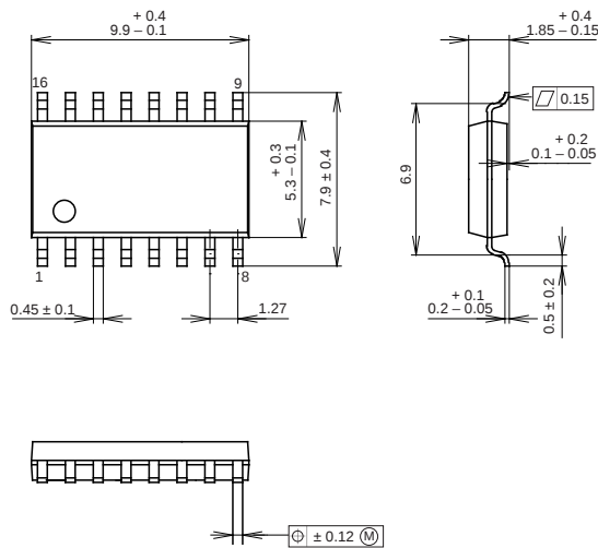
16PIN SOP (PLASTIC) 300mil
