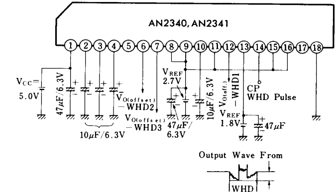
Test Circuit 7 ( V_{O(Offset)}-WHD1\sim3 )
