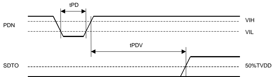
Power-down &amp; Reset Timing
