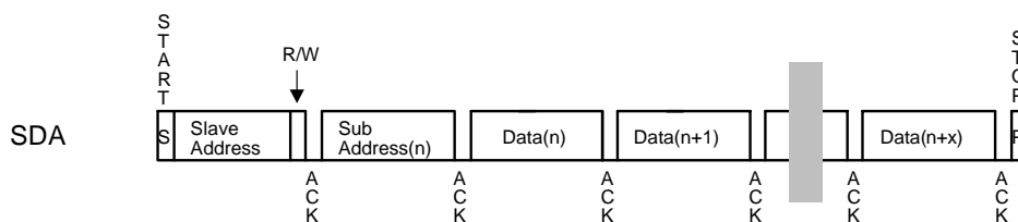
Figure 13. Data transfer sequence at the I 2 C-bus mode
