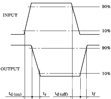
WAVEFORMS
