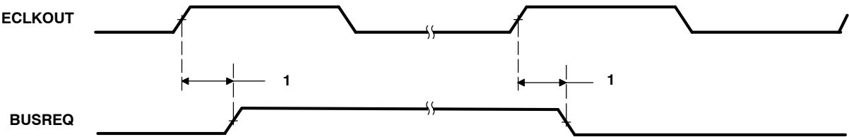
Figure 37. BUSREQ Timing
