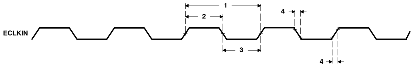
Figure 23. ECLKIN Timings
