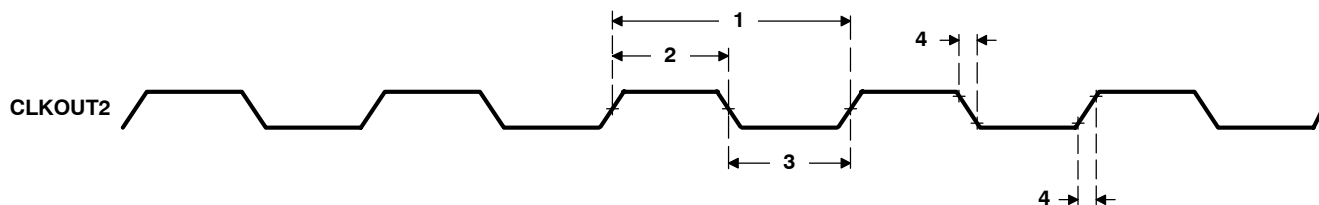
Figure 20. CLKOUT2 Timings [C6711/11B]
