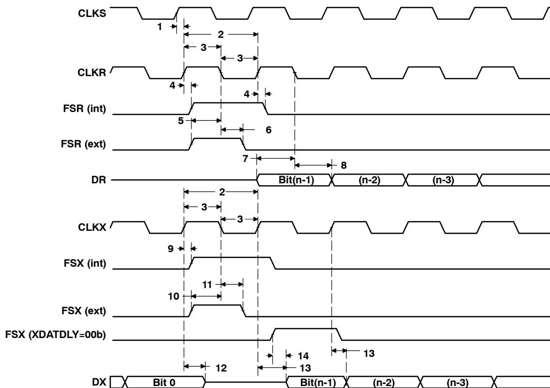
Figure 45. McBSP Timings
