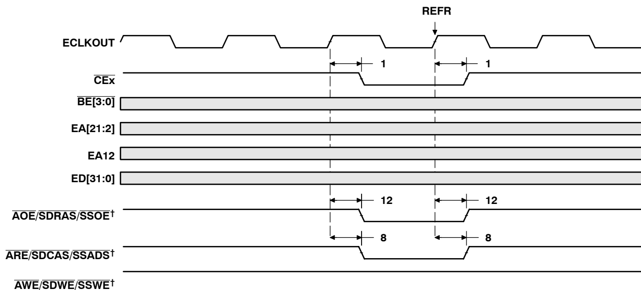
Figure 33. SDRAM DEAC Command
