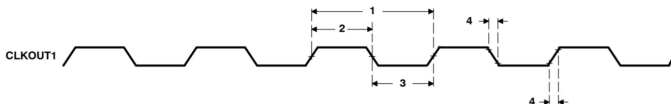
Figure 19. CLKOUT1 Timings [C6711/11B Only]
