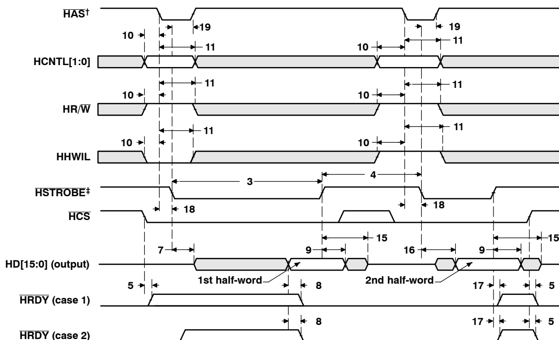
Figure 42. HPI Read Timing (HAS Used)
