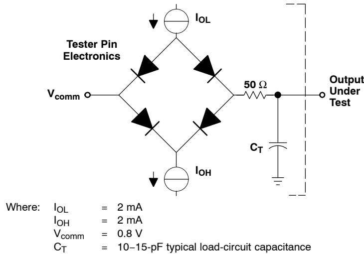
Figure 13. Test Load Circuit for AC Timing Measurements for C6711/C6711B Only
