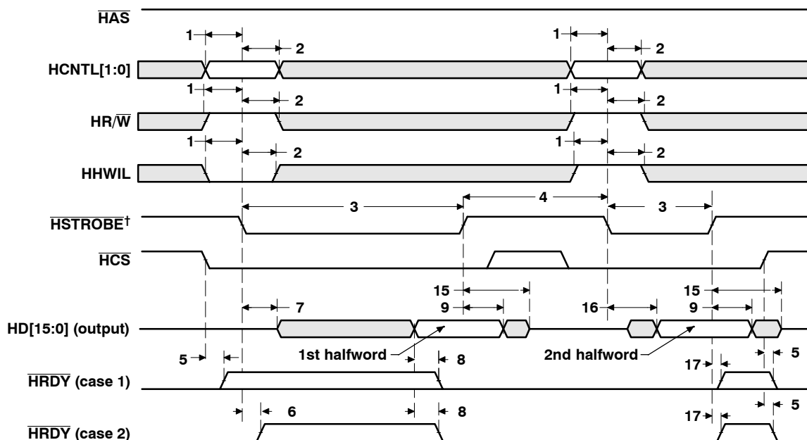
Figure 41. HPI Read Timing (HAS Not Used, Tied High)
