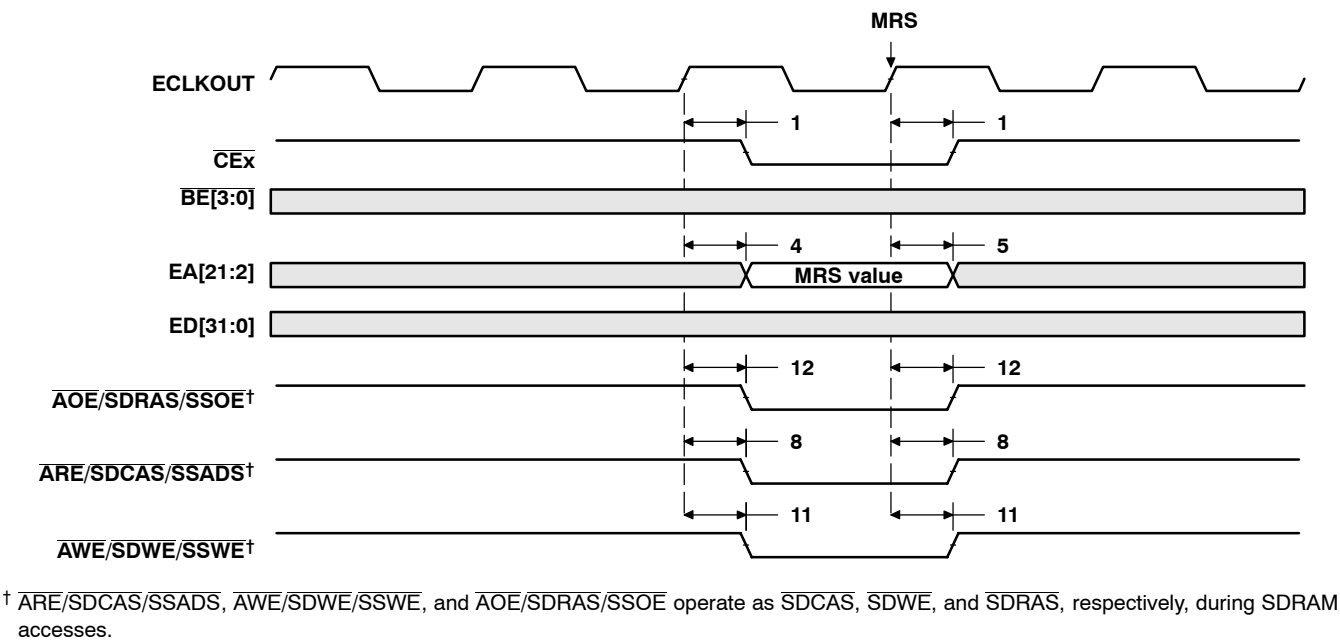
Figure 35. SDRAM MRS Command
