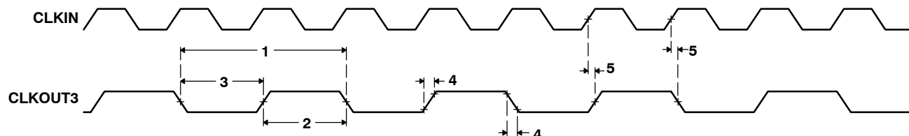
Figure 22. CLKOUT3 Timings [C6711C Only]
