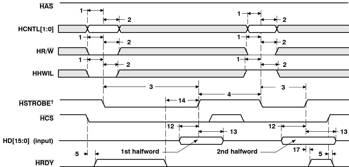
Figure 43. HPI Write Timing (HAS Not Used, Tied High)
