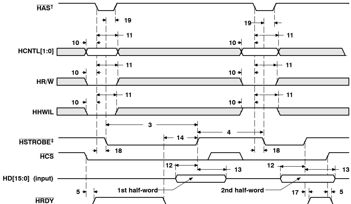
Figure 44. HPI Write Timing (HAS Used)
