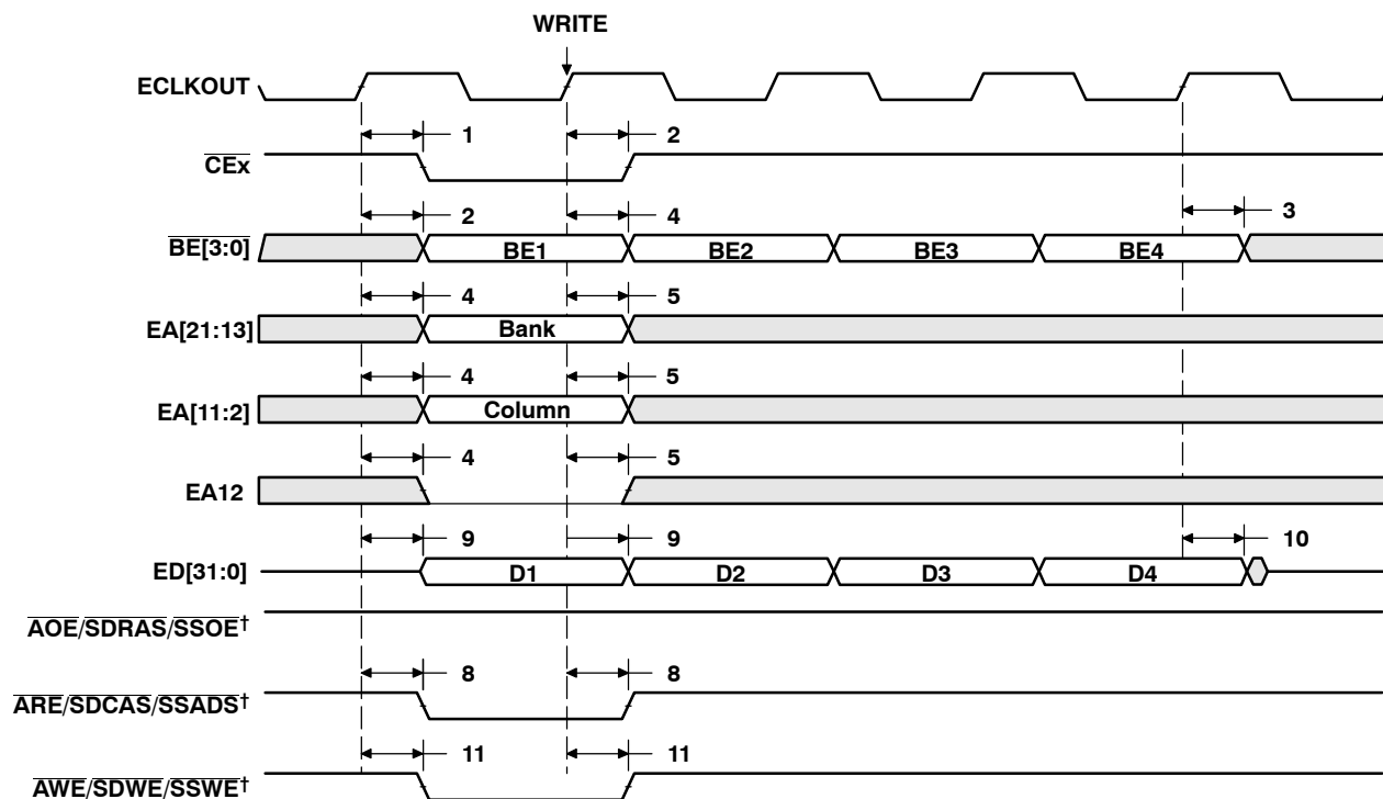
Figure 30. SDRAM Write Command
