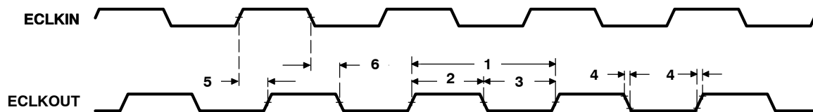
Figure 24. ECLKOUT Timings
