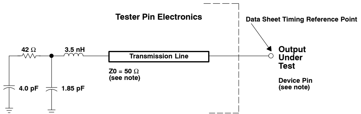
Figure 13. Test Load Circuit for AC Timing Measurements for C6711/C6711B Only
