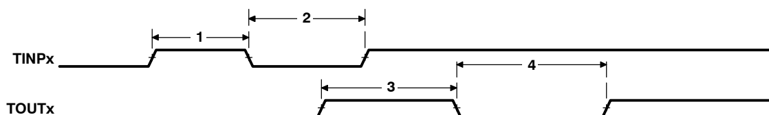
Figure 51. Timer Timing
