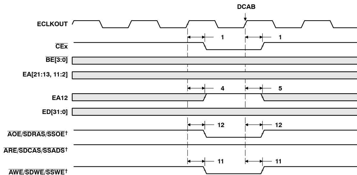
Figure 31. SDRAM ACTV Command
