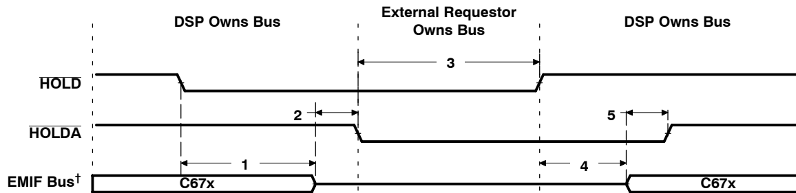
Figure 36. \overline{\text{HOLD}}/\text{HOLDA} Timing
