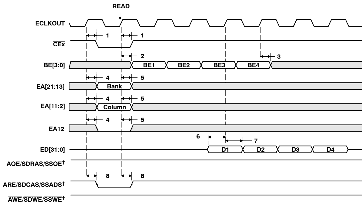
Figure 29. SDRAM Read Command (CAS Latency 3)
