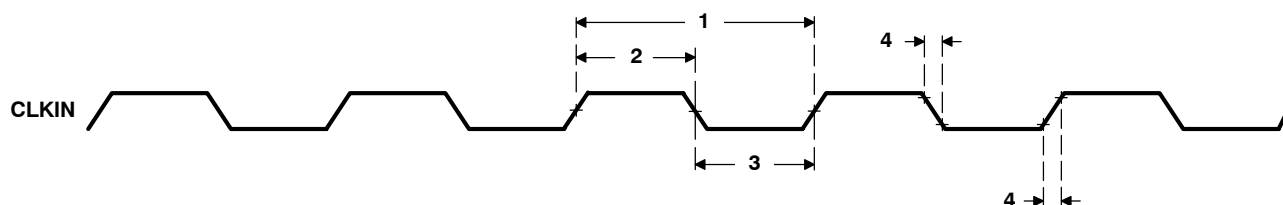
Figure 18. CLKIN Timings
