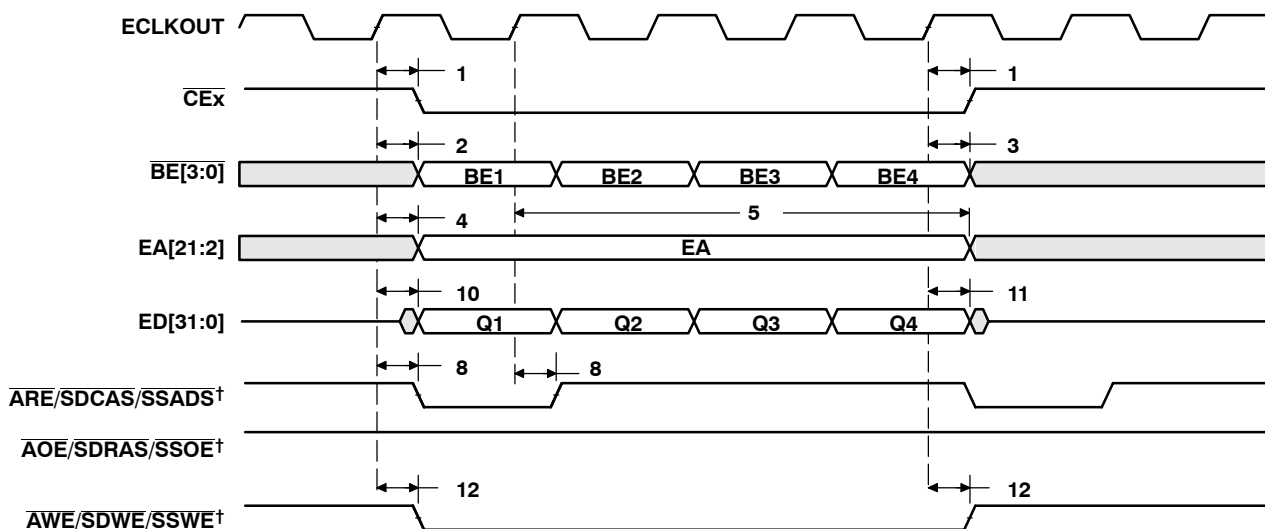
Figure 27. SBSRAM Read Timing
