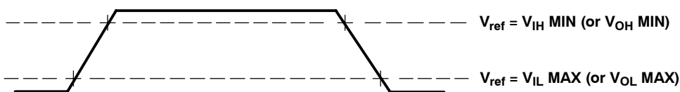
Figure 16. Rise and Fall Transition Time Voltage Reference Levels
