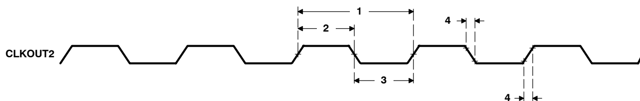
Figure 21. CLKOUT2 Timings
