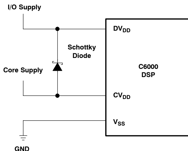
Figure 12. Schottky Diode Diagram
