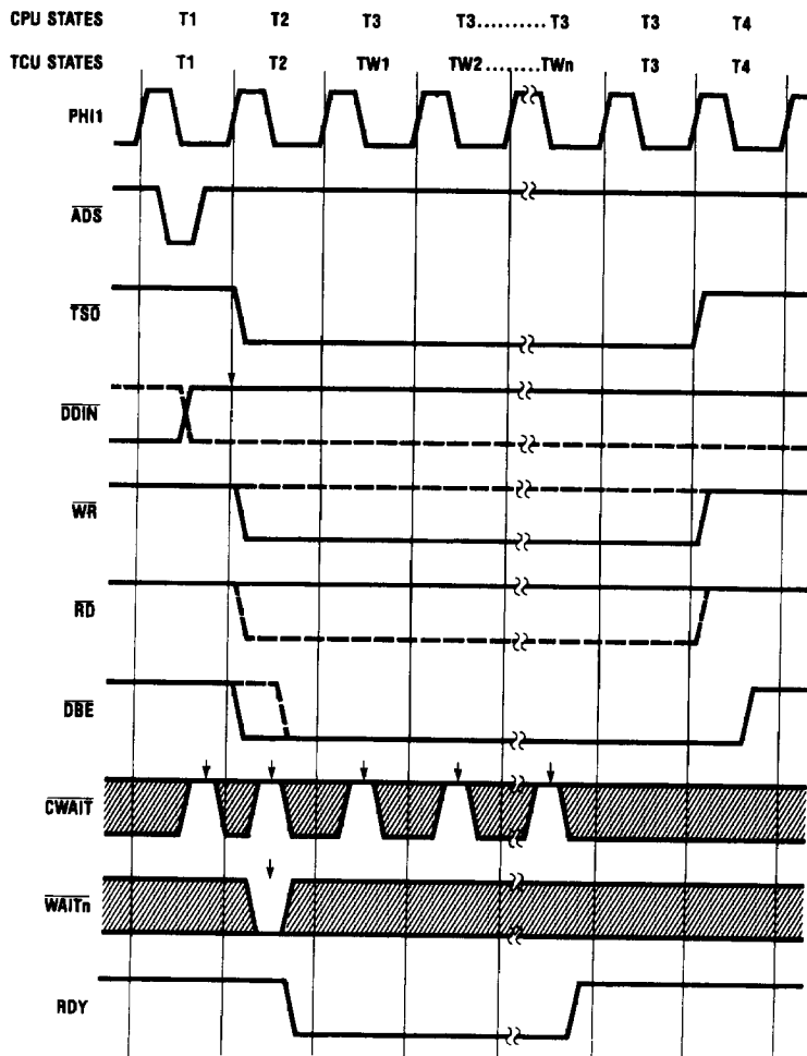
FIGURE 1-9. Wait State Insertion Using WAIT n (Fast Cycle)
