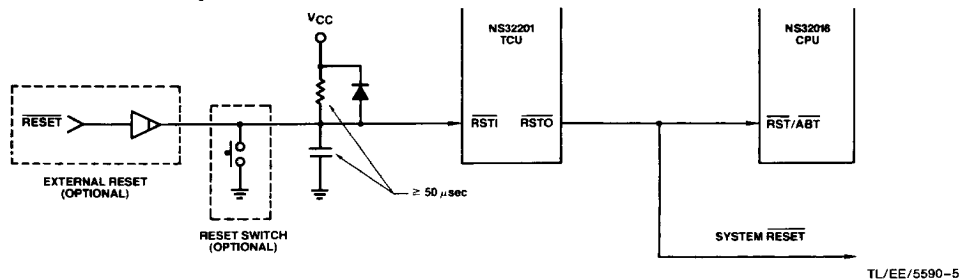
FIGURE 1-3a. Recommended Reset Connections (Non Memory-Managed System)
