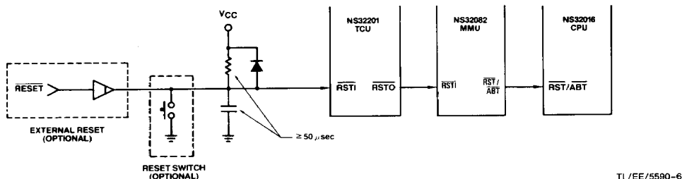
FIGURE 1-3b. Recommended Reset Connections (Memory-Managed System)
