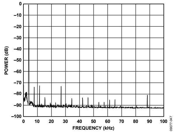
Figure 15. Power vs. Frequency, f_{MCLK} = 16 MHz, f_{OUT} = 3.8 kHz, Frequency Word = 0x000FBA9
