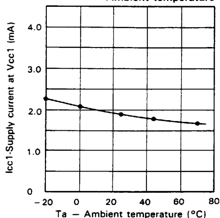
Supply current at Vcc1 vs. Ambient temperature
