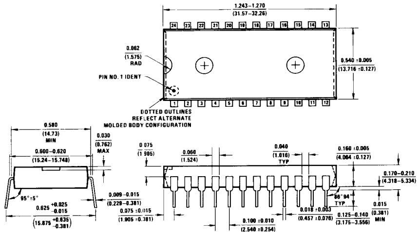
24-Lead Molded Dual-in-Line Package (N) Order Number COP621C-XXX/N, COP641C-XXX/N, COP821C-XXX/N or COP841C-XXX/N NS Package Number N24A
