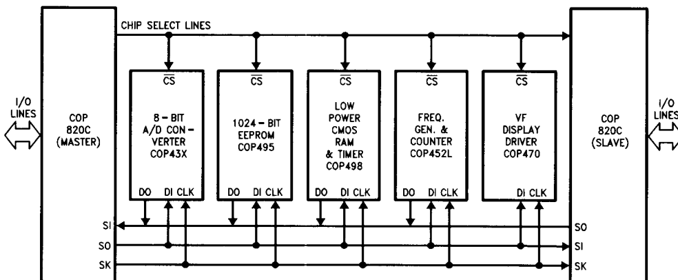
FIGURE 8. MICROWIRE/PLUS Application
