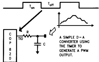
FIGURE 11. Timer Application
