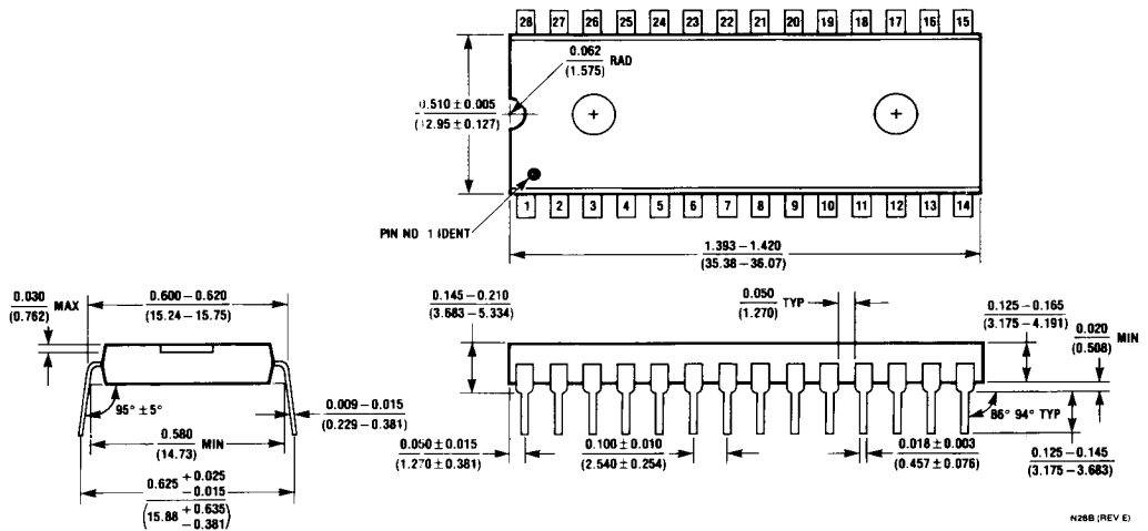
28-Lead Molded Dual-in-Line Package (N) Order Number COP620C-XXX/N, COP640C-XXX/N, COP820C-XXX/N or COP840C-XXX/N NS Package Number N28B
