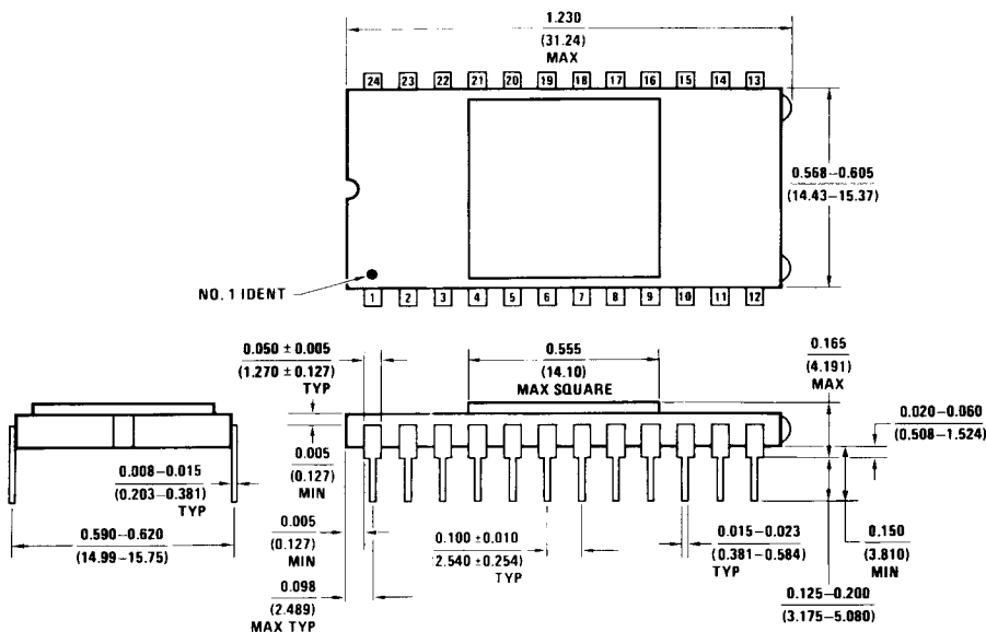
24-Lead Hermetic Dual-in-Line Package (D) Order Number COP821C-XXX/D or COP841C-XXX/D NS Package Number D24C
