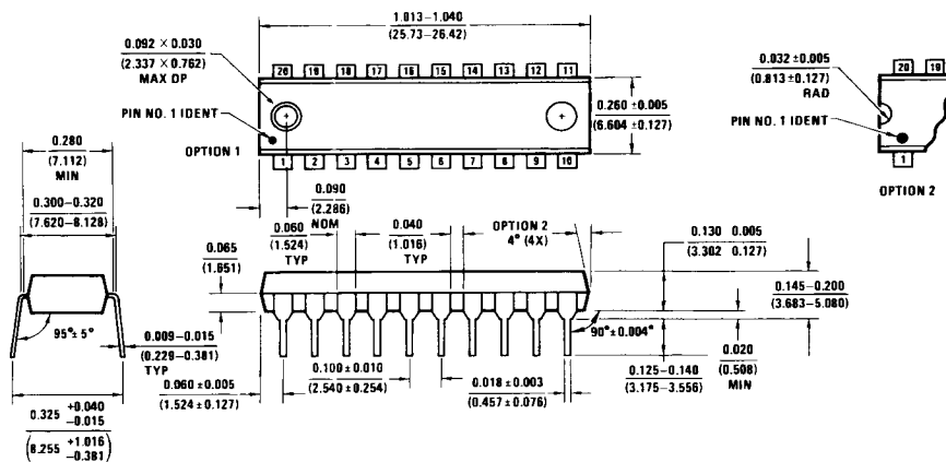
20-Lead Molded Dual-in-Line Package (N) Order Number COP622C-XXX/N, COP642C-XXX/N, COP822C-XXX/N or COP842C-XXX/N NS Package Number N20A
