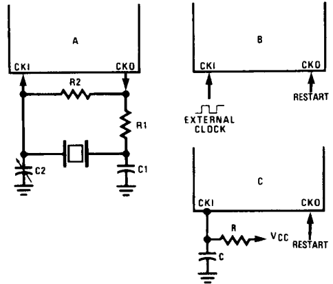
FIGURE 5. Crystal and R-C Connection Diagrams
