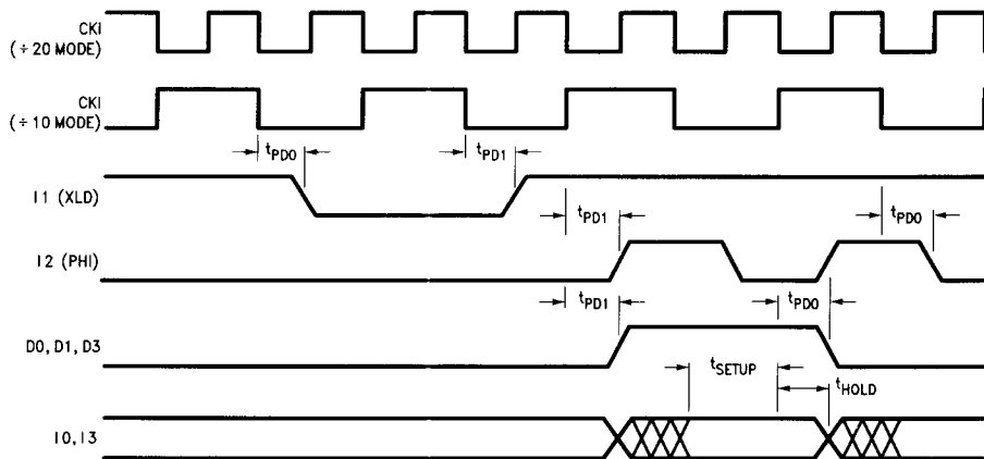
FIGURE 2a. AC Timing Diagrams in ROMless Mode
