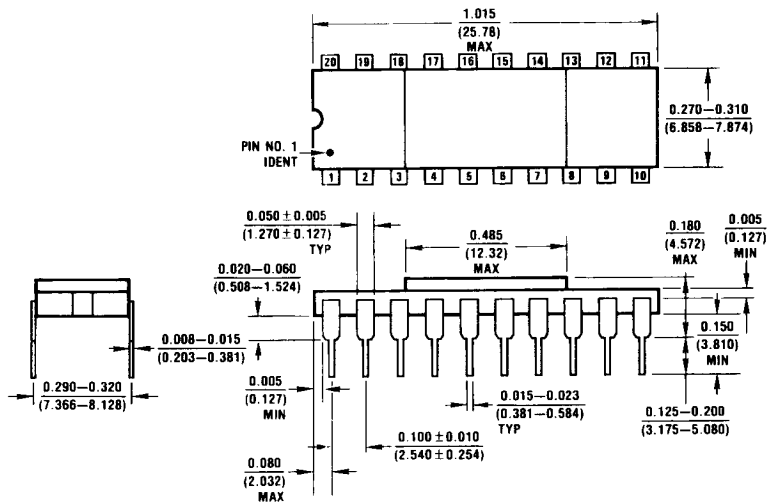
20-Lead Hermetic Dual-in-Line Package (D) Order Number COP822C-XXX/D or COP842C-XXX/D NS Package Number D20A
