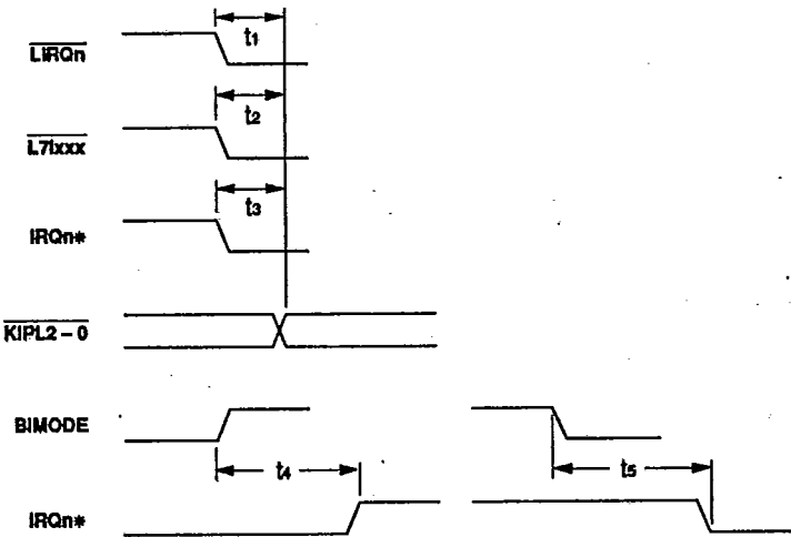
Figure 6 : INTERRUPT SIGNAL TIMING a) IPL Generation, BI-MODE Effect on IRQ Generation
