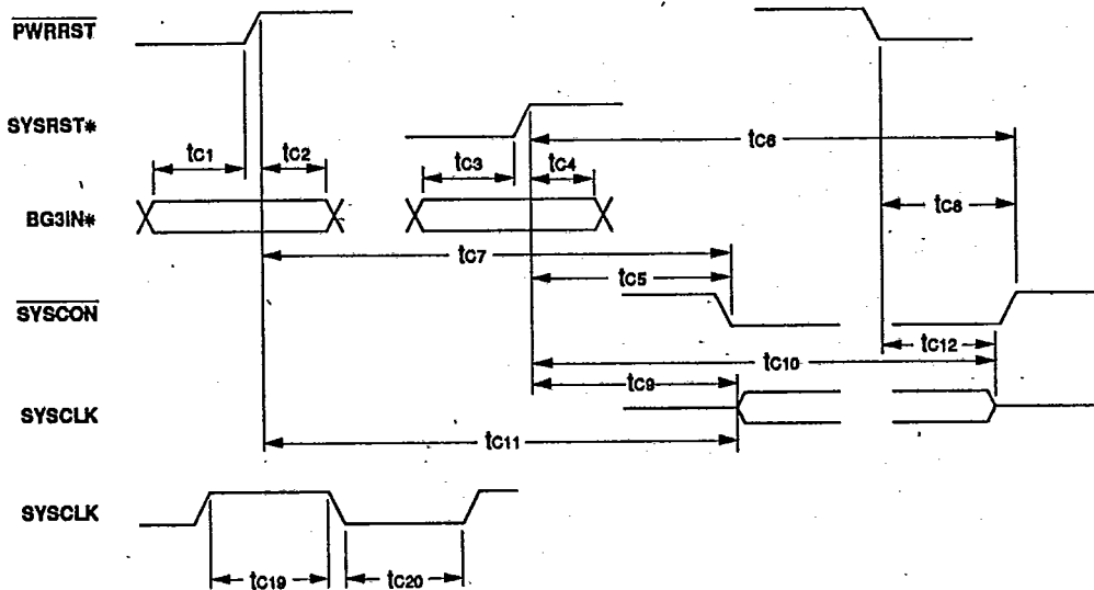
Figure 5 : SYSCON and BI-MODE™ TIMING
