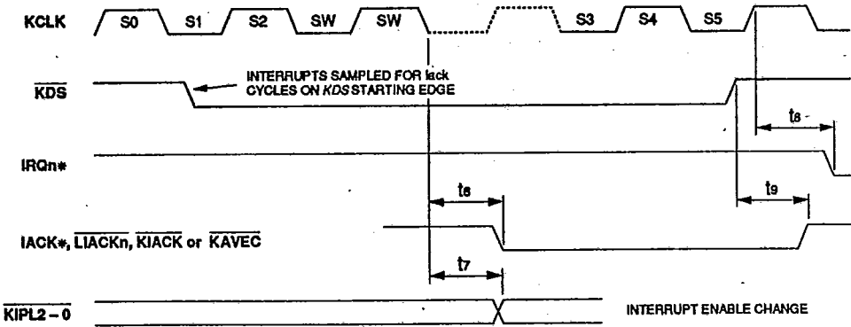
b) IRQ Assertion, Interrupt Enabling and Acknowledging
