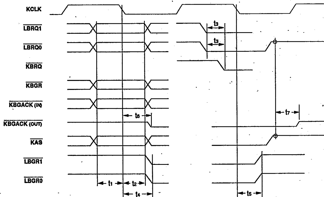
Figure 8 : LOCAL BUS REQUESTER TIMING
