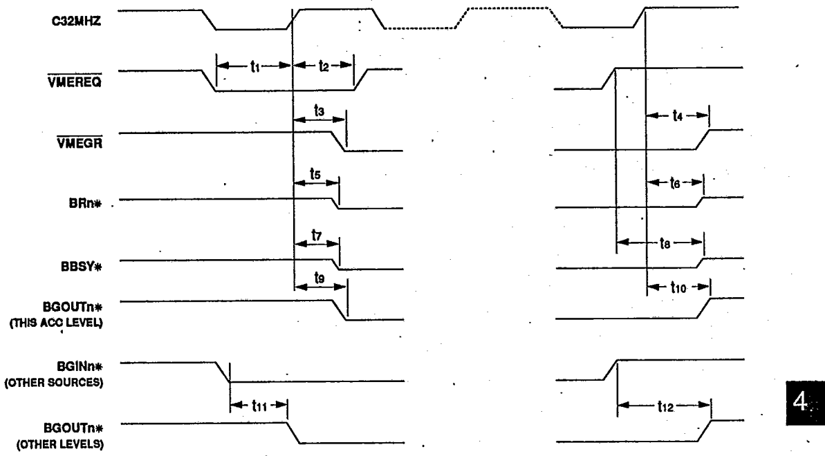
Figure 9 : VMEbus REQUESTER TIMING
