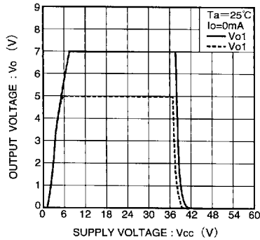
Fig.9 Output voltage vs. supply voltage (typ.)
