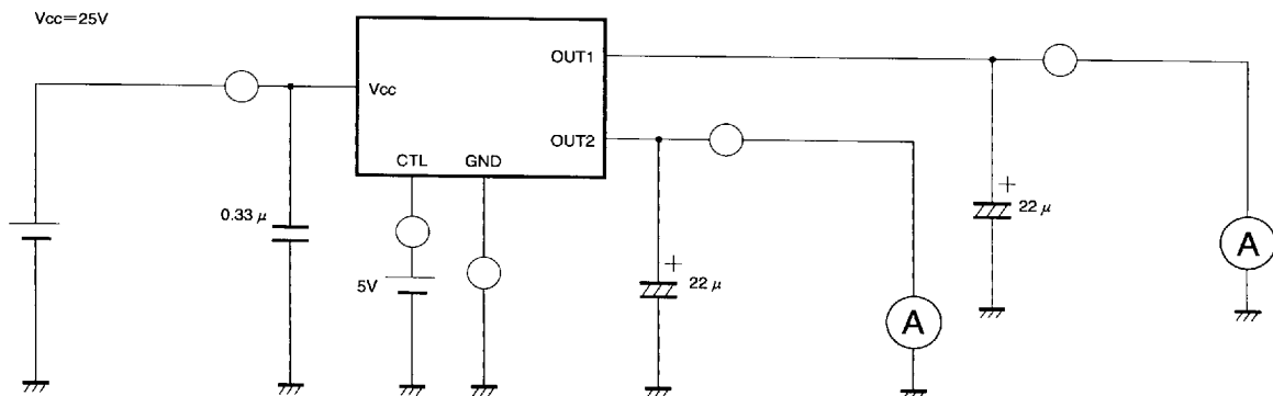
Fig.4 Circuit for measuring bias current and standby circuit current
