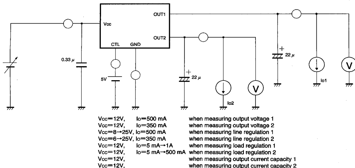
Fig.1 Circuit for measuring output voltage, line regulation, load regulation, and output current capacity
